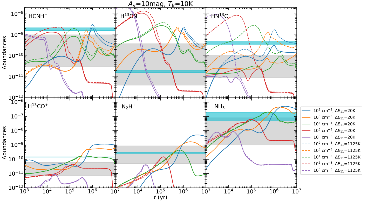
Fig. 19. Molecular abundances relative to H_2 as a function of time, estimated from Chempl (Du 2021). The different colors correspond to the different H_2 number densities, from 10^2 \text{ cm}^{-3} to 10^6 \text{ cm}^{-3} . The solid and dashed lines represent the modeling results with the energy barrier \Delta E_{11} = 20 \text{ K} and \Delta E_{11} = 1125 \text{ K} for reaction (11), respectively. The observed molecular abundances in our studies are indicated by the gray shaded regions, while the molecular abundances in TMC1 (Agúndez & Wakelam 2013) are indicated by the cyan shaded regions.
