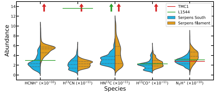
Fig. 11. Comparison of the fractional abundances of different species with respect to H_2 determined on a pixel-by-pixel basis. The y -axis has been divided by the scaling values, which are given in parentheses after the molecule names along the x -axis for better visualization. The dotted lines indicate the 25%, 50%, and 75% percentiles of the respective distributions. The molecular abundances in TMC1 and L1544 are also indicated for comparison. The arrows indicate that their abundances are higher than the maximum value on the y -axis.
