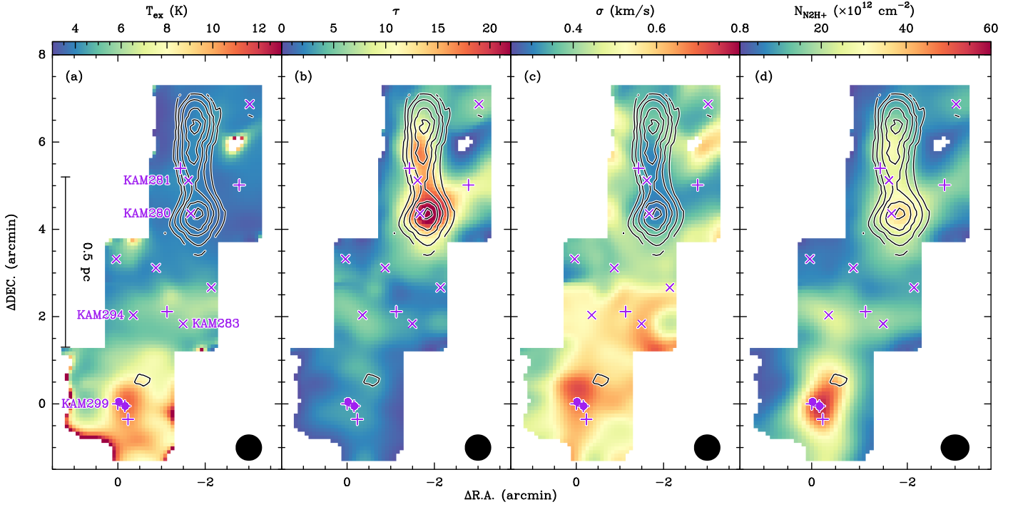
Fig. 9. Distributions of the fitted properties of N_2H^+ (1–0) in Serpens South. (a) N_2H^+ (1–0) excitation temperature, (b) total optical depth, (c) velocity dispersion, and (d) N_2H^+ column density. The red pixels at the southern boundary of panel a have large uncertainties for the fitted excitation temperatures. The overlaid HCNH^+ (2–1) integrated-intensity contours are the same as in Fig. 2a.
