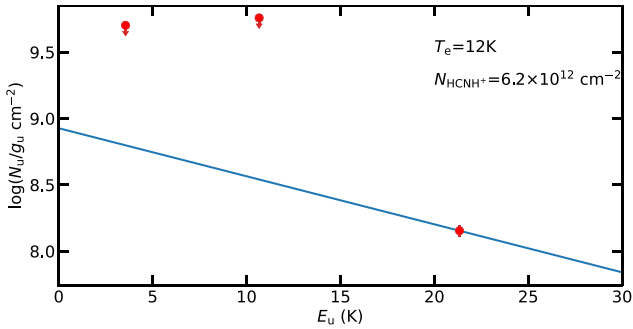
Fig. 10. Population diagram of HCNH^+ toward KAM299. The blue line represents the fit expected from the excitation temperature and HCNH^+ column density, which are given in the top-right corner.
