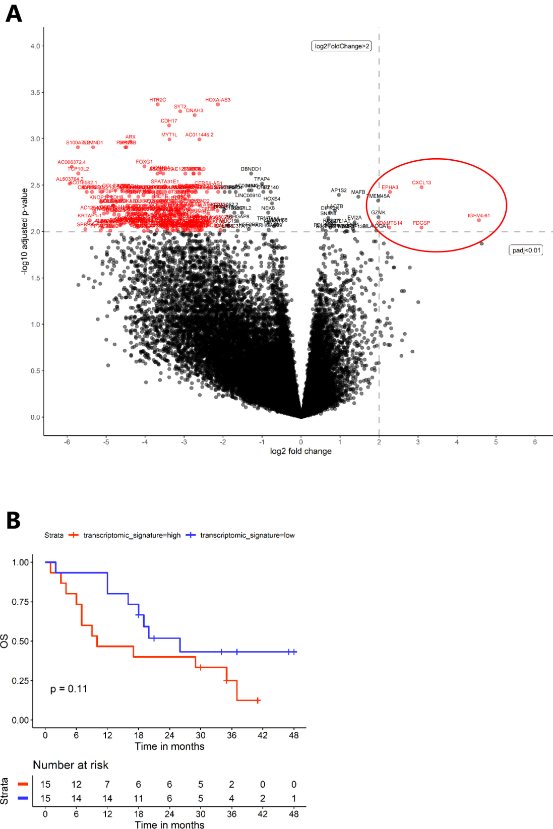
Figure 4 Transcriptomic characterization of the papillary renal cell carcinoma tumor microenvironment subtypes defined by IHC. (A) Volcano plot representing the messenger RNAs differential-expression analysis (=32,378 genes) from DESeq2, between the two groups identified from IHC in the AXIPAP trial cohort (n=30). Under the condition of log 2 (fold-change) >2 and p adjusted <0.01, five differentially overexpressed genes were identified between the two groups (red circle). (B) Kaplan-Meier survival curves (overall survival (OS)) according to subgroups with a “high transcriptomic signature” and “low transcriptomic signature”, defined as a median of the five significant differentially overexpressed genes. IHC, immunohistochemistry.
