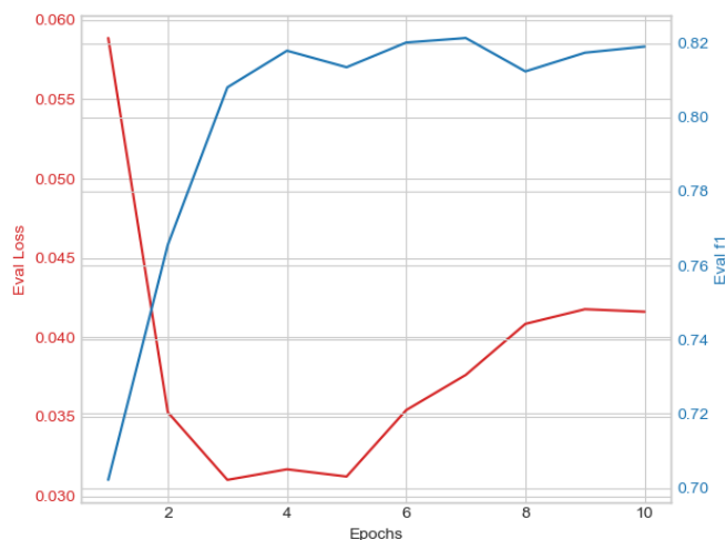
Figure 1: BERT Fine-tuning
