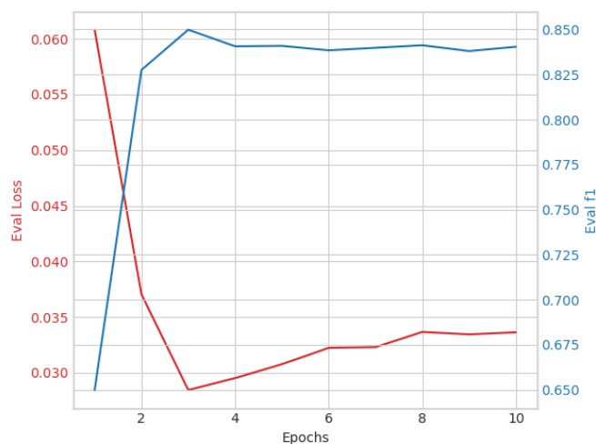
Figure 2: XLM-RoBERTa Fine-tuning
