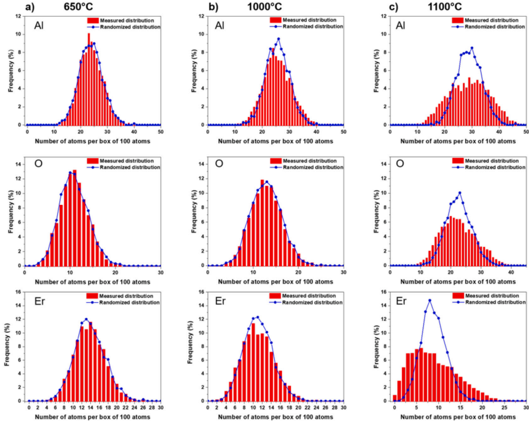
Fig. 7. Frequency distributions of Al, O and Er observed in the case of a distribution of 100 atoms in layers annealed at (a) 650 °C, (b) 1000 °C and (c) 1100 °C.
