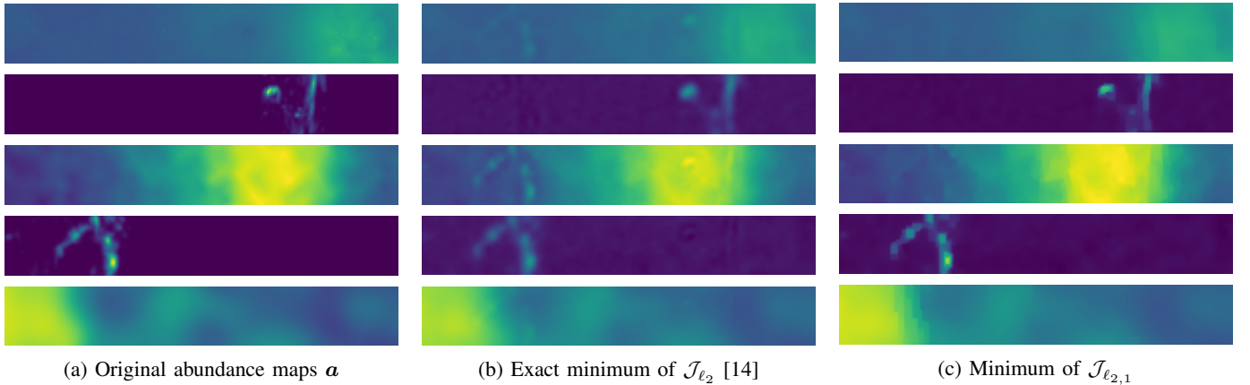
Fig. 6: Comparison between original abundance maps \mathbf{a} , on the left, and the ones reconstructed with the explicit minimization of \mathcal{J}_{\ell_2} and with the fast minimization of \mathcal{J}_{\ell_{2,1}} , where \text{SNR}_{\text{dB}} = 30 dB for both MS and HS input datasets. Each of these abundance maps is associated in order with the spectra of Fig. 2. All maps share the same dynamic range.
