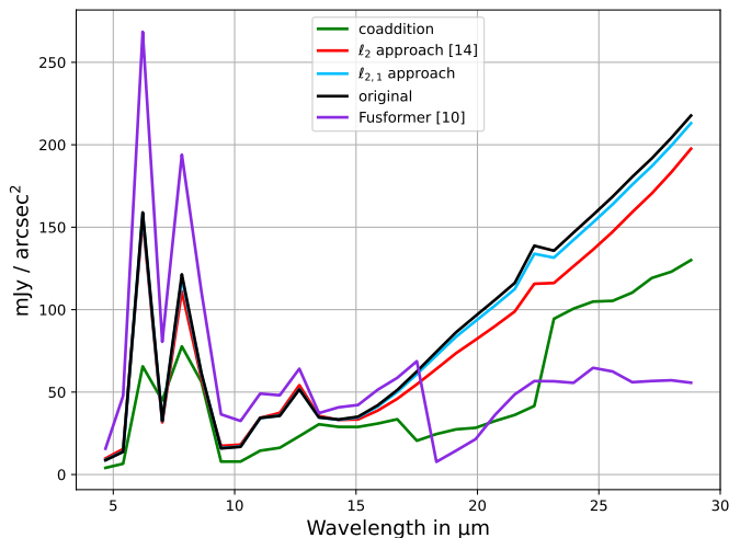
Fig. 9: Example of spectra reconstructed with the coaddition, the \ell_2 [14] and the \ell_{2,1} approaches, and Fusformer [10] for the same spatial position, taken in a high gradient region. SNR of input datasets: 40 dB.
