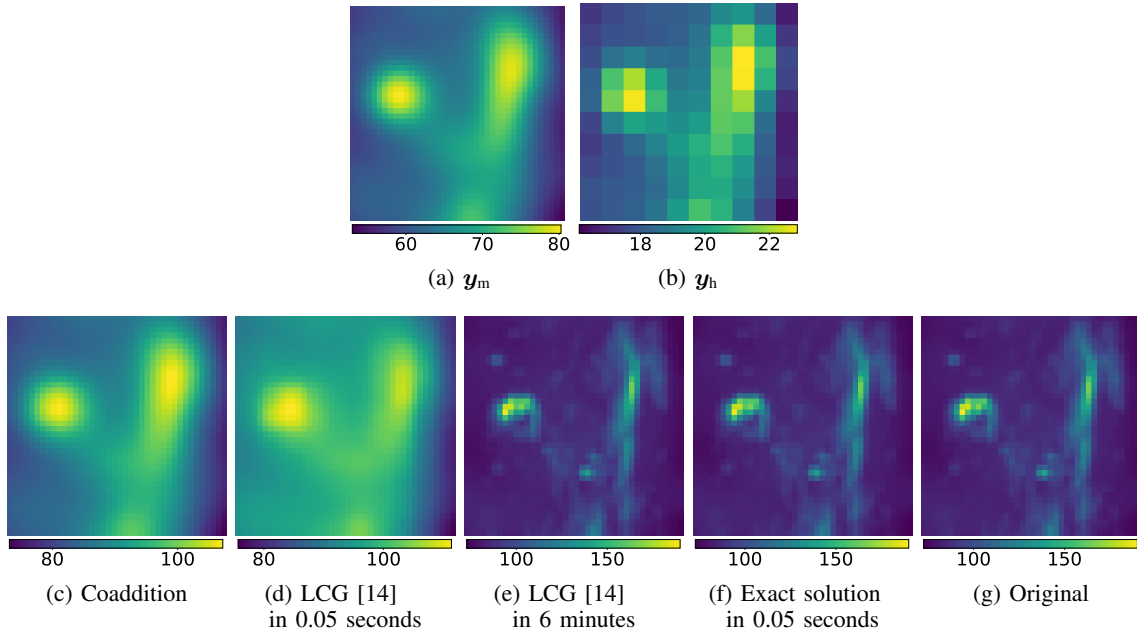
Fig. 4: Imagery data \mathbf{y}_m and spectrometry data \mathbf{y}_h with \text{SNR}_{\text{dB}} = 100 dB on top, and reconstruction with the coaddition method Fig. 4c. The next figures show results of the minimization of \mathcal{J}_{\ell_2} with the LCG algorithm in 0.05 second and 6 minutes (value of criterion at 0.1% of \min(\mathcal{J}_{\ell_2}) ), and with the demonstrated explicit method (section III-B) in 0.05 seconds. The last figure is the original image. Central wavelength for all images is 25.5 \mu\text{m} . Unit is \text{mJy arcsec}^{-2} . The dynamical scales for the three last figures are identical.
