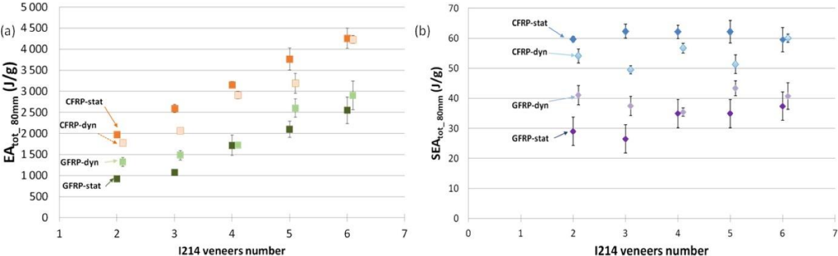
Figure 47. Evolution of (a) EA tot_80 mm (b) SEAtot_80 mm according to the number of poplar layers, the nature of the skins (CFRP: Carbon Fiber Reinforced Polymer; GFRP: Glass Fiber Reinforced Plastic), and static and dynamic conditions. Reproduced from [199]
