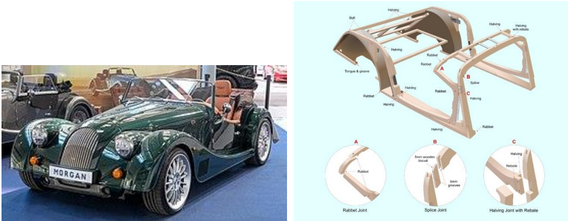
Figure 61: The last model of Morgan cars, the “Morgan Plus Six” and its ash frame structure [231, 233].
