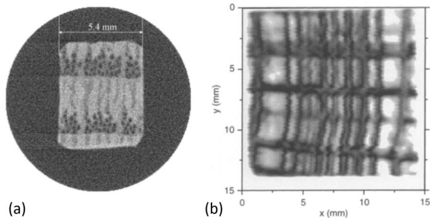
Figure 33: (a) X-ray CT image (28.3 keV, spatial resolution = 0.1 mm) of an oak ( Quercus rubra L.) sample 0, and (b) THz image (spatial resolution = 0.3-0.5 mm) of a beech ( Fagus sylvatica L.) sample 0
