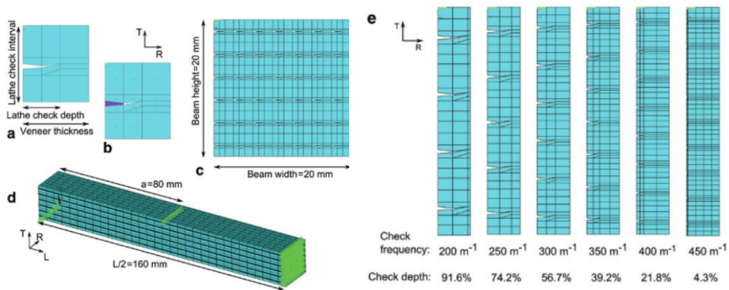
Figure 39 – Finite element model of an LVL beam. (a) Base Pattern; (b) base pattern with glued cracks (the glue is purple in color); (c) beam cross-section (crack frequency 300\ m^{-1} ); (d) half of the beam (the green triangular symbols represent the boundary conditions); (e) finite element model of the six cracked veneers used in the numerical model [120].
