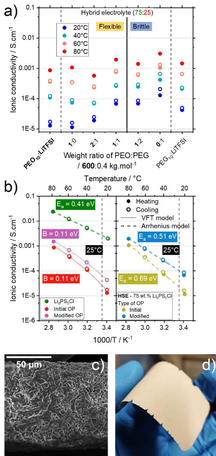
Figure 4: Combination of high and low molar mass PEO in high-loading ceramic HSE. (a) Effect of PEO:PEG ratio to HSE ionic conductivity in temperature. (b) Activation mechanism for precursors and 75 wt.% ceramic HSEs. Initial organic phase (OP): \text{PEO}_{10}:\text{LiTFSI} – Modified OP: (\text{PEO}:\text{PEG} = 1:1 \text{ (w)})_{10}:\text{LiTFSI} . (c) SEM picture of the optimized HSE cross-section. (d) Image of the large area optimized HSE membrane.
