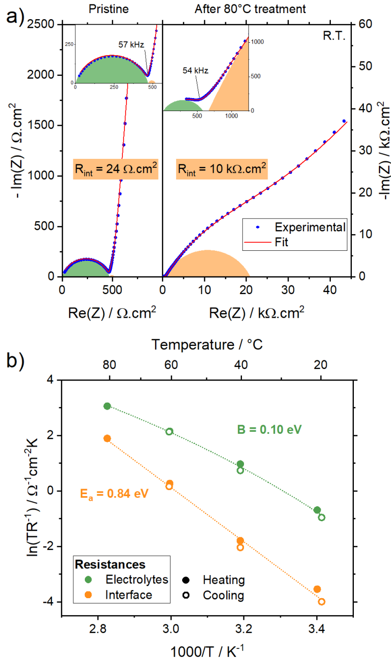
Figure 6: Compatibility of ceramic and polymer phases probed by EIS. (a) EIS spectra of trilayer PEO 10 :LiTFSI | Li 6 PS 5 Cl | PEO 10 :LiTFSI before and after 80°C treatment. (b) Evolution of R_{\text{elec}} and R_{\text{int}} in temperature and their related activation energies.
