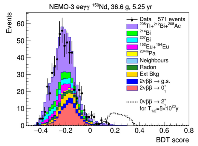
Fig. 13 BDT distribution for the 0\nu\beta\beta decay to the 2_1^+ excited state
