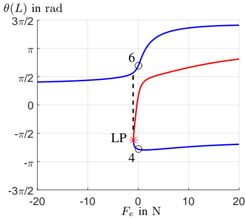
Fig. 4: Stability analysis of a TDCR composed of one disk at the tip, actuated with T_1 = 32\text{ N} and deformed by increasing the external tip force magnitude F_e . The tip force orientation is \phi = -\pi/8 and the disk radius is r_d = 2\text{ mm} . Stable and unstable robot configurations are represented in blue and red resp. A Limit Point (LP) bifurcation is detected, indicated by a red star.
