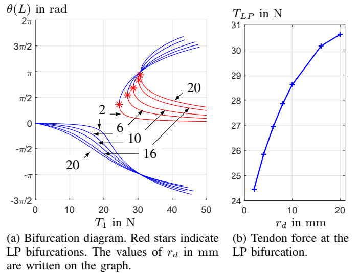
Fig. 5: Evolution of the bifurcation diagram according to the disk radius.
