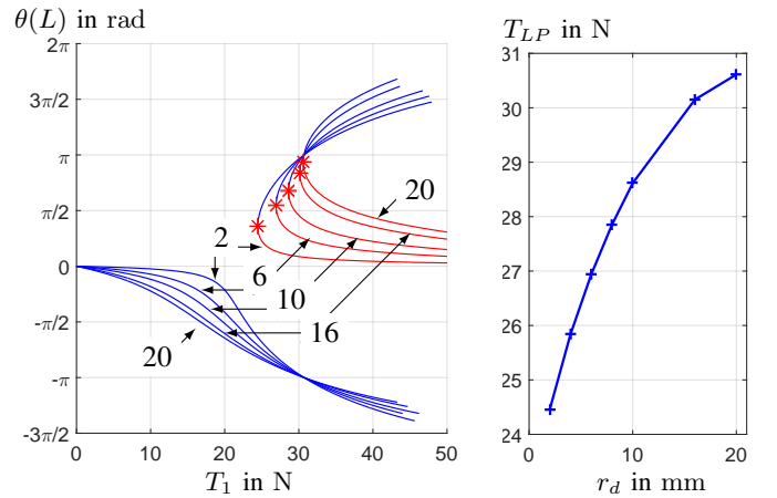
(a) Bifurcation diagram. Red stars indicate LP bifurcations. The values of r_d in mm are written on the graph. (b) Tendon force at the LP bifurcation.
