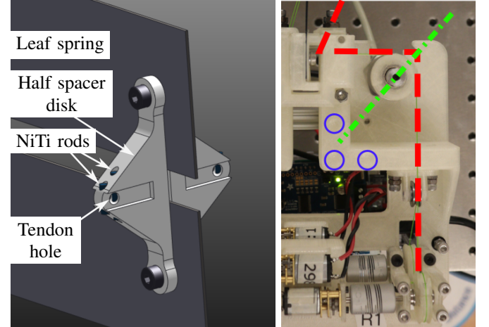
(b) CAD view of a spacer disk.
