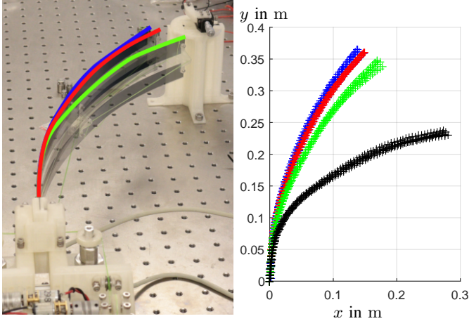
(a) Overlay of robot configurations. (b) Measured backbone position.
