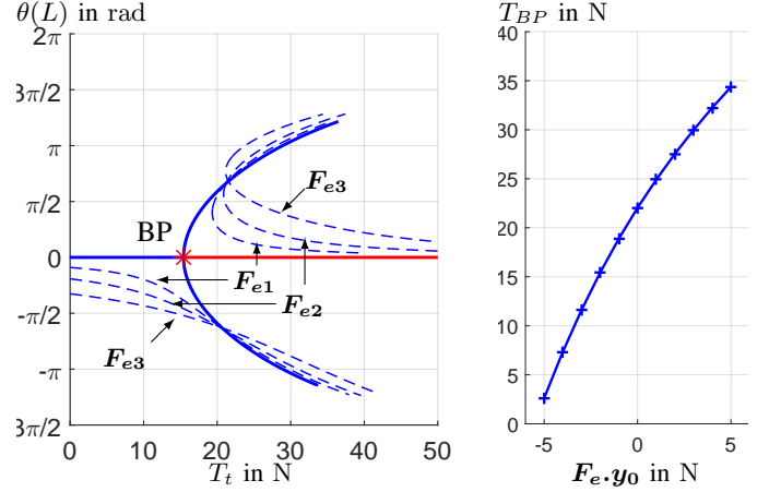
(a) Bifurcation diagrams considering different tip forces \mathbf{F}_e : (F_e, \phi) : plain line \mathbf{F}_e = (2, \pi/2) , and dashed lines \mathbf{F}_{e1} = (2.16, 5\pi/8) , \mathbf{F}_{e2} = (2.83, 3\pi/4) , \mathbf{F}_{e3} = (5.23, 7\pi/8) (b) Tendon force at the BP bifurcation.
