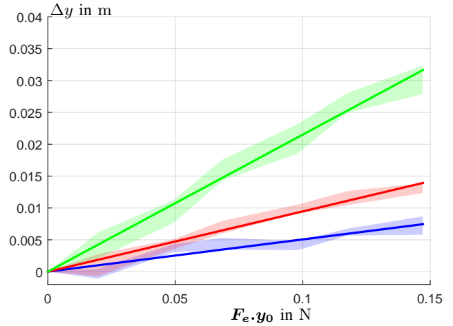
Fig. 18: Displacement to tip force relation for different values of total tendon force applied on the backbone and for \theta(L) = -\pi/4 . The distributions of the measured values for each tip force amongst the 5 trials are represented with blue, red, and green areas. Plain thick lines represent the linearized relationship.
