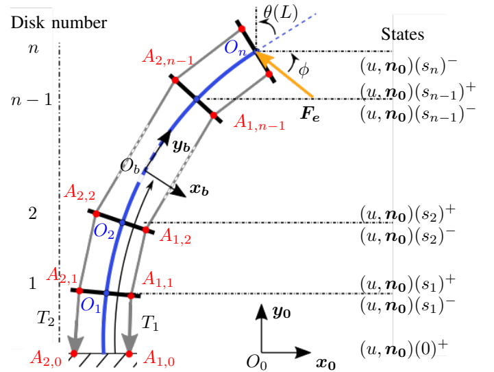
Fig. 1: Schematics of the planar TDCR. The elastic backbone is represented in blue, the tendons in grey and the disks in black. The tendon holes are depicted with red dots. The robot is subject to an external force applied on its tip represented in orange.
