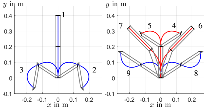
(b) Robot shapes for configurations 1 to 6. (c) Robot shapes for configurations 7 to 12.
