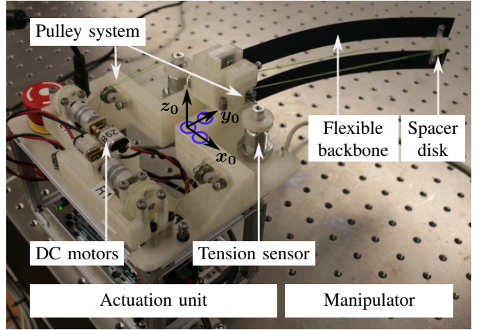
(a) Experimental setup. The robot is composed here of one disk.
