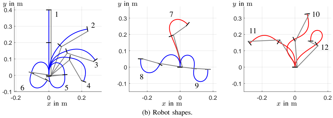
Fig. 10: Stability analysis of a TDCR composed of two disks and deformed by increasing the tendon tension T_1 . Stable and unstable robot configurations are represented in blue and red resp. Limit Point (LP) bifurcations are detected, indicated by a red stars. On the right side, a subset of robot shapes are represented, the actuated tendon being plotted in grey.
