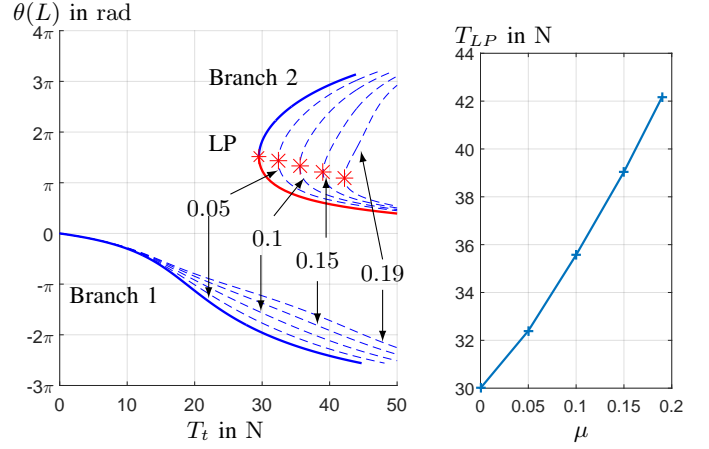
(a) Bifurcation diagrams considering different values of \|\mu\| , written on the graph. Solid lines: diagram without friction. (b) Tendon force at the LP bifurcation.
