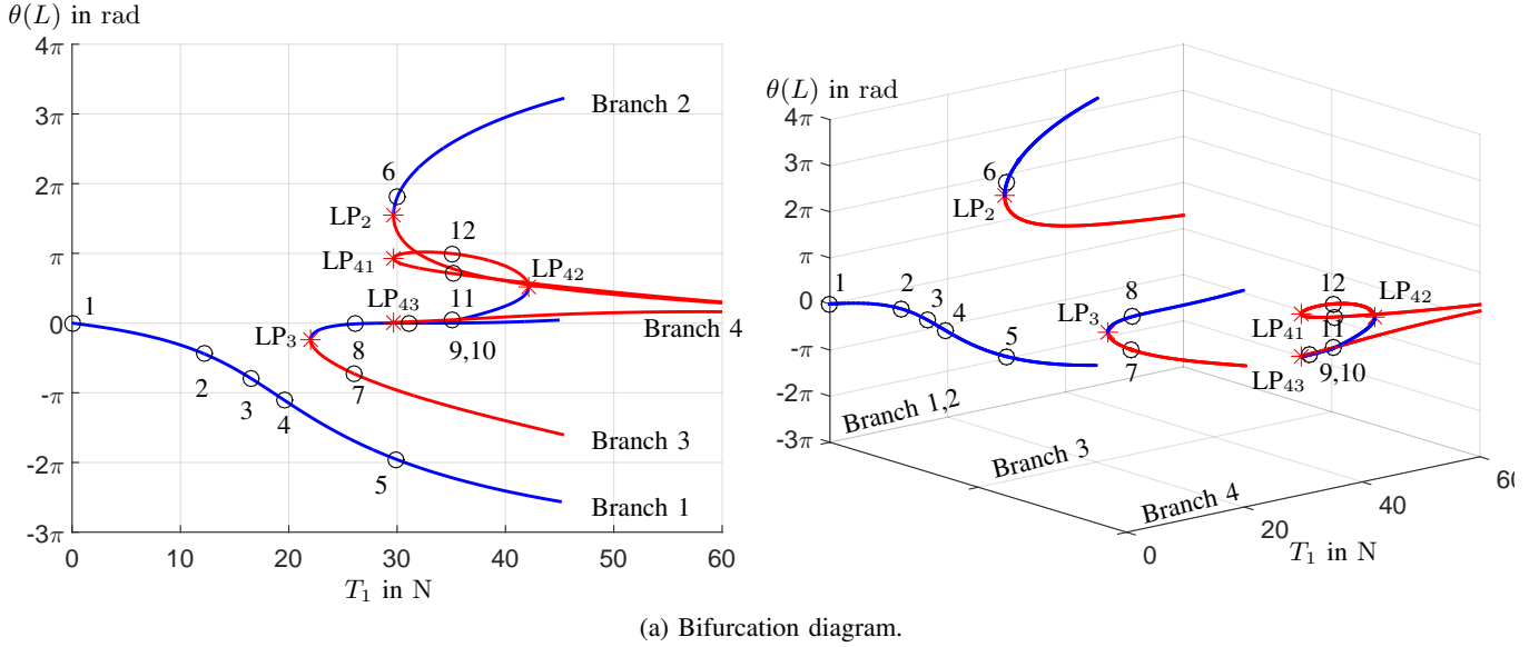
(a) Bifurcation diagram.
