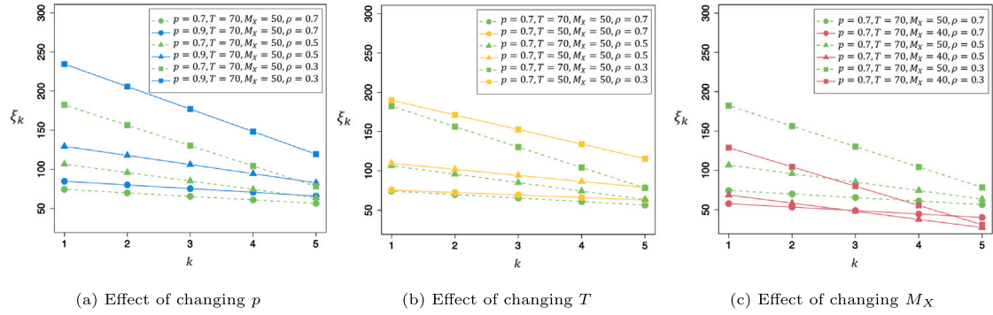
Fig. 2. Effect of changing decision variables on \xi_k for three different values of \rho = 0.3, 0.5, 0.7 . The parameter set considered here is \alpha = 0.1, \lambda_1 = \lambda_2 = 0.7 and the failure threshold is L = 60 .
