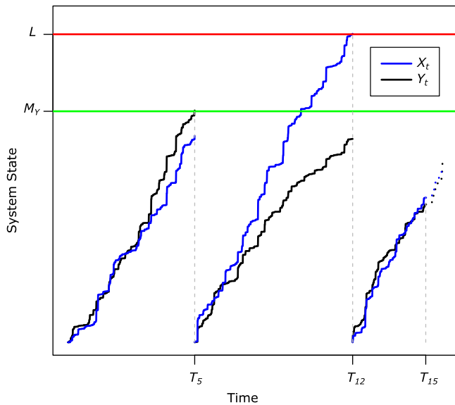
Fig. 1. Schematic evolution of a maintained system state under CMP.
