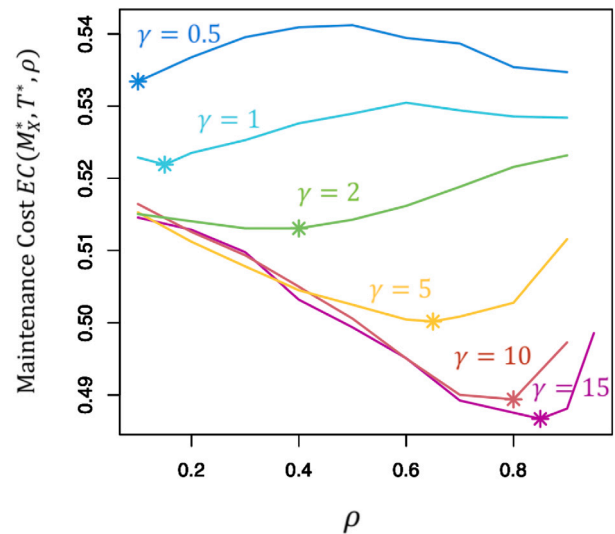
Fig. 4. CMP maintenance cost as a function of \rho for different values of \gamma .
