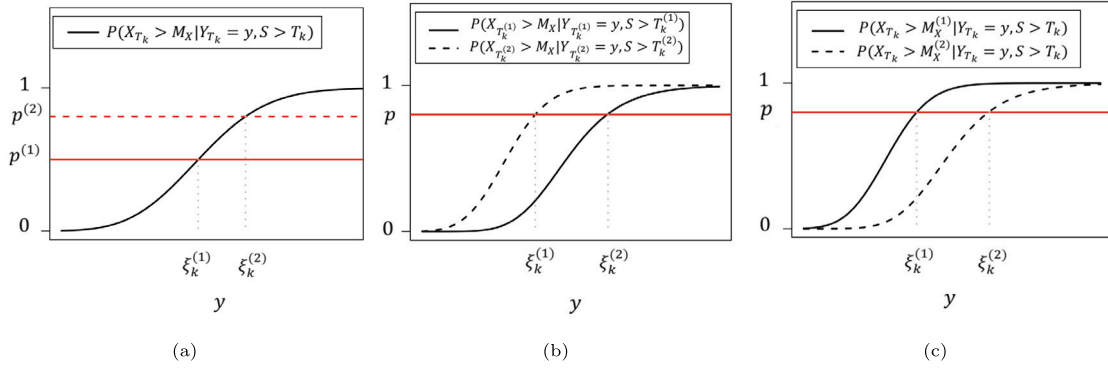
Fig. B.5. Conditional probability and adaptive threshold for IMP as a function of decision variables.
