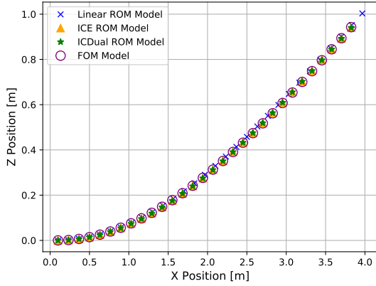
Fig. 4: Comparison of the nonlinear static solution between the nonlinear FOM and the different ROMs.
