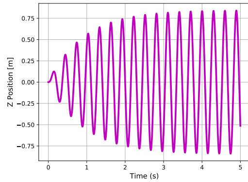
Fig. 6: Temporal axial and vertical displacements of the tip of the beam.
