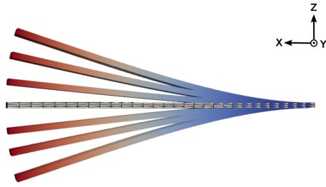
Fig. 5: Nonlinear FOM displacements over a period.
