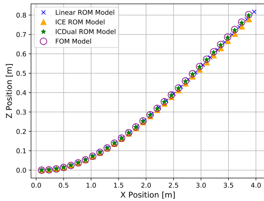
Fig. 7: Comparison of the maximal displacements in periodic regime between the FOM and the different ROM solutions. The beam is subjected to a vertical sinusoidal load at the tip of amplitude 2500 N and frequency 3.38 Hz.
