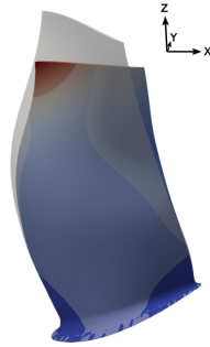
Fig. 15: First dual mode of the blade, determined from the three first linear normal modes around the prestressed position at 2750 rpm.
