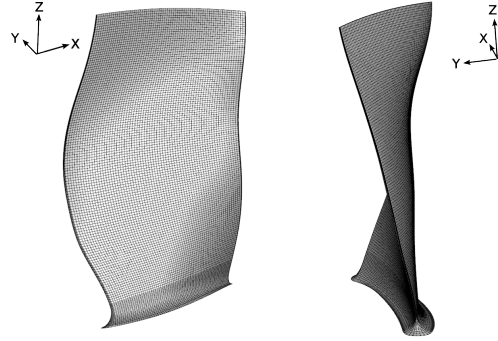
Fig. 12: Mesh of the blade.
