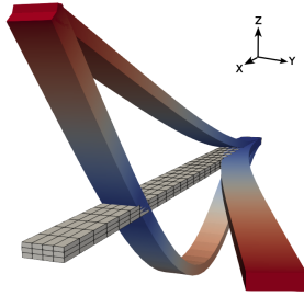
Fig. 1: Visualization of the first 3 linear normal modes of the beam at 0 rpm. The mesh is the initial geometry.
