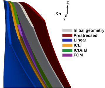
Fig. 17: Comparison between the FOM and the ROM solutions under the opposite of the static load (12).
