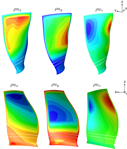
Fig. 18: Steady aerodynamic forces on the suction side (top) and the pressure side (bottom) of the blade.
