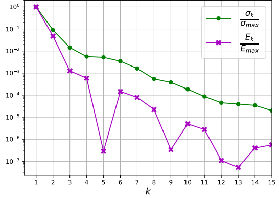
Fig. 2: Normalized singular values (green) and linearized strain energy (purple) of the modes obtained by the SVD of the matrix of residuals.
