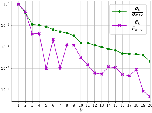
Fig. 8: Normalized singular values (green) and linearized strain energy (purple) of the SVD modes of the beam in rotation at 500 rpm.
