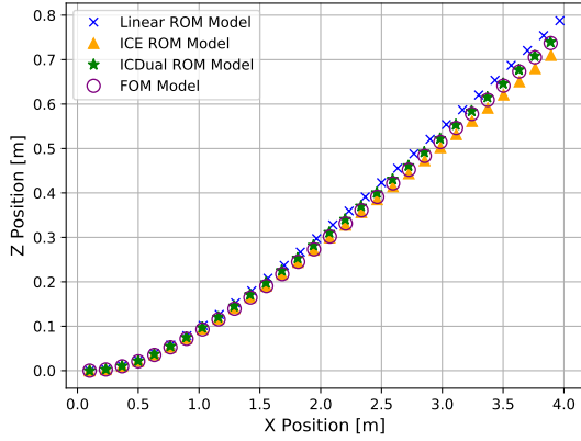
Fig. 10: Comparison of the maximal displacement in periodic regime between the FOM and the different ROM solutions. The beam is subject to a vertical sinusoidal load at the tip, of amplitude 7350 N and frequency 9.67 Hz.
