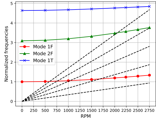
Fig. 13: Campbell of the blade for the first 3 structural modes.
