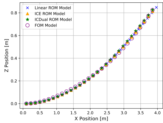
Fig. 9: Comparison of the static deflections between the FOM and the different ROMs. The beam is in rotation at 500 rpm subject to a vertical static load at the tip of 210000 N.
