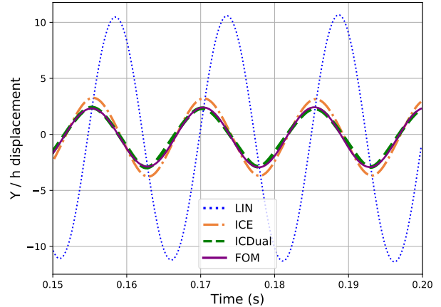
Fig. 19: Time response of the tip trailing edge along the Y direction.
