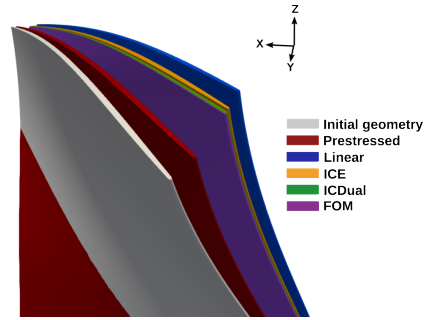
Fig. 16: Comparison between the FOM and the ROM solutions under the static load (12).
