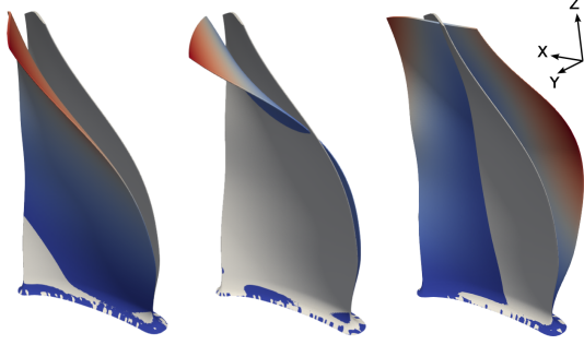
Fig. 14: First 3 linear normal modes (1F, 2F and 1T) of the blade at 2750 rpm.
