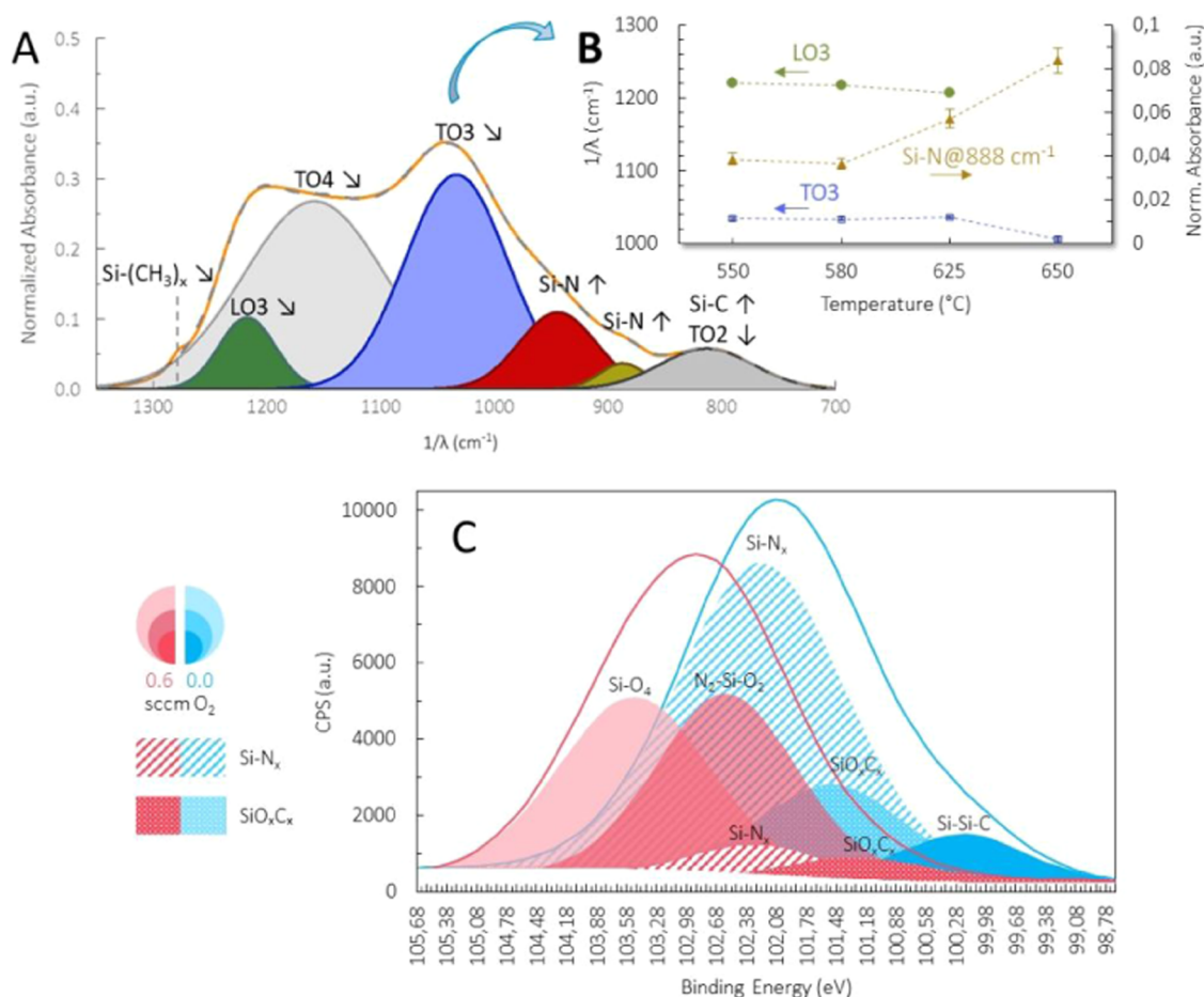
Figure 6. Structural and microscopic characteristics of \text{SiO}_x\text{N}_y films. (A) FT-IR fingerprint domain, with deconvolution of overlapping absorptions for a film processed at 625\text{ }^\circ\text{C} at 0.3\text{ O}_2/\text{BMDSD} ratio. Trends with increasing T_d : shifts are indicated by \rightarrow\leftarrow and changes in intensity by \downarrow\uparrow arrows. (B) Peak position in wave numbers for LO3, TO3, and Si-N bands as a function of T_d at 0.3\text{ O}_2/\text{BMDSD} ratio. (C) XPS Si 2p deconvolution analysis for two \text{SiO}_x\text{N}_y samples processed at 650\text{ }^\circ\text{C} with 0.3\text{ O}_2/\text{BMDSD} , and 550\text{ }^\circ\text{C} with 0.0\text{ O}_2/\text{BMDSD} ratios.
