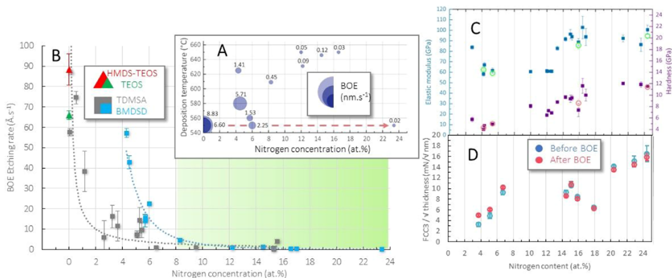
Figure 5. Functional properties of SiO_xN_y films. (A) BOE rate as a function of the nitrogen content and T_d . (B) BOE etching rate of SiO_xN_y from BMDSD (light blue squares), TDMSA 27 (gray squares), and SiO_2 and SiO_x films processed at 550 °C from TEOS 13 (green triangle) and HMDS-TEOS 15 (red triangle), respectively. Power trend lines were added for visual aid. (C) Elastic modulus (blue squares) and hardness (purple squares). Red and green open circles refer to values after BOE. (D) Critical force of delamination for SiO_xN_y films from BMDSD before and after BOE. Films in panels (C and D) were processed at T_d 550 °C.
