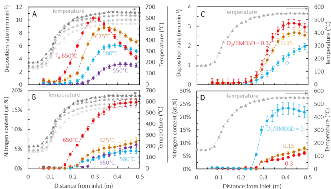
Figure 4. Parametric analysis of SiO_xN_y deposition. (A) Deposition rate and (B) nitrogen content in SiO_xN_y films produced for various T_d , at a 0.3 O_2/BMDSD flow ratio. The temperature profiles in the reactor are shown as gray data, with the lightest to the darkest corresponding to the lowest up to the highest T_d . (C) Deposition rate and (D) nitrogen content for SiO_xN_y films produced for variable O_2/BMDSD flow ratios, at T_d 550 °C. The temperature profile of T_d 550 °C is shown in the gray data. All four diagrams are presented as a function of the distance from the inlet; i.e., the position of each Si coupon.
