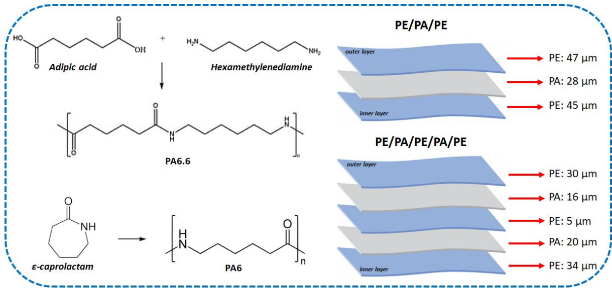
Figure 1. Chemical structure of polyamide 6, polyamide 6.6, their monomers, composition of multilayer PE and PA films and their respective thicknesses.
