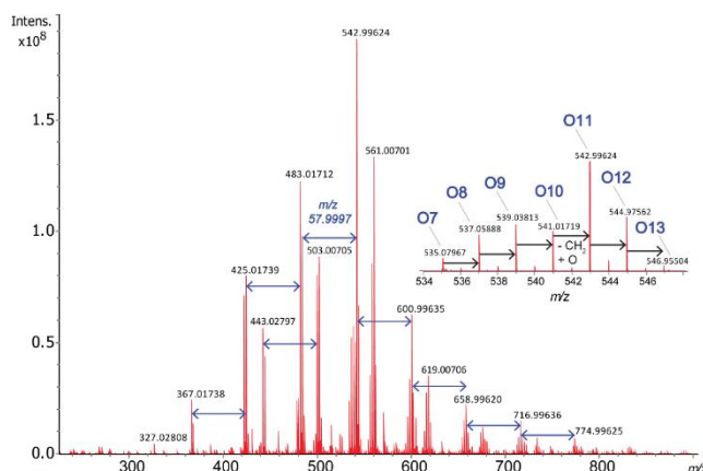
Figure 3. piASAP FTICR mass spectrum of MMAO-12 showing ions series separated by 57.999 u ( \text{CH}_3\text{AlO} ). The zoomed areas showcase distribution of \text{Al}_8\text{O}_y ( y = 7, 8, 9, 10, 11, 12 and 13 ). MMAO-12 clusters in piASAP FTICR mass spectrum of MMAO-12 in mass range ( m/z 534–547).
