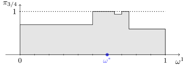
Figure 10: Preferential information corrected with \ell -out-of- k repair algorithm in Example 9
