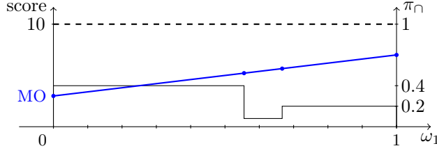
Figure 7: Overlap of the unnormalized possibility distribution \pi_\cap from Example 8 with the score of the alternative MO
