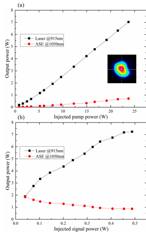
Fig. 3. Output powers at 915 nm and 1050 nm of the 30/125 LMA fiber amplifier injected through a MFA, (a) versus pump power for an injected signal power of 450 mW and (b) versus injected signal power for an injected pump power of 23 W. In black: laser power at 915 nm; in red: forward ASE power at 1050 nm; Insert: signal beam profile at the maximum output power.
