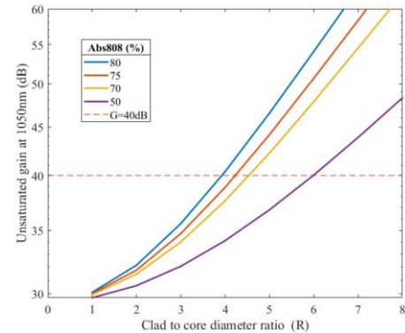
Fig. 1. Unsaturated gain at 1050 nm calculated from eq. 1 and eq. 3 as a function of clad-to-core diameter ratio R for a fixed gain at 915 nm of 20dB and for an unsaturated pump absorption varying between 50% and 80%.
