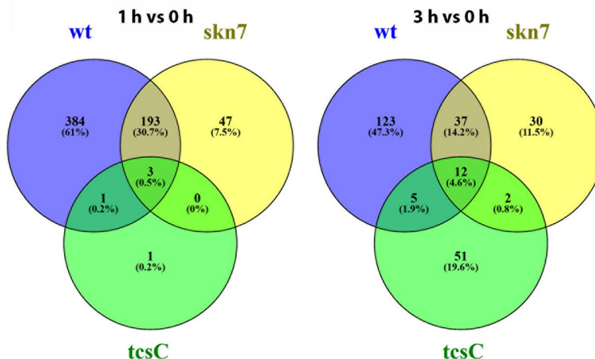
Fig. 4 Venn diagrams showing differentially expressed genes of the three strains in response to fludioxonil (threshold value: 1.5 log 2 FC). wt Wild type strain AfS35, tcsC \Delta tcsC and skn7 \Delta skn7 mutant
