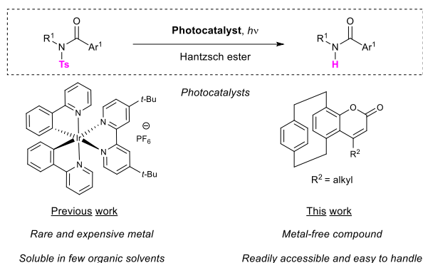
Scheme 1. Examples of catalytic photodesulfonation reactions
