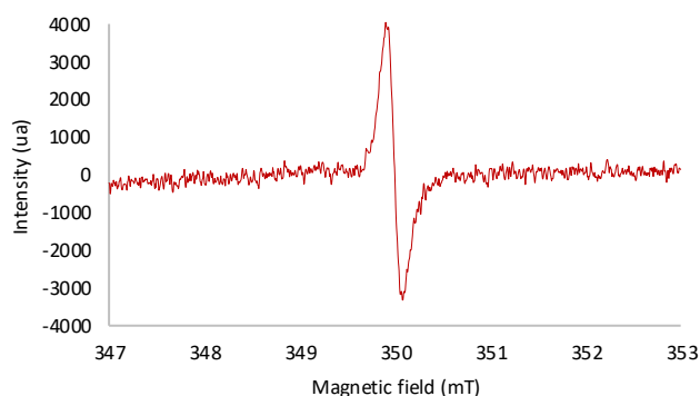
Figure 1. EPR spectroscopy of a solution of 3a (5 mol %), 4a (1 equiv.) and 7 (1.2 equiv.) in \text{CH}_2\text{Cl}_2 (0.05 M) under irradiation at 300 nm in a quartz tube under an argon atmosphere.
