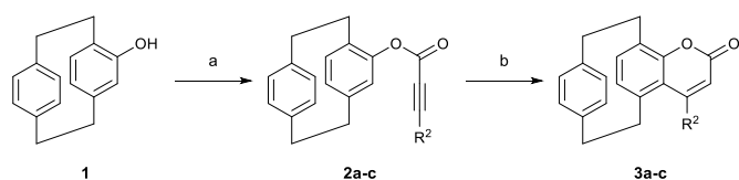
Scheme 2. Synthesis and spectroscopic properties of pCp-based coumarins
