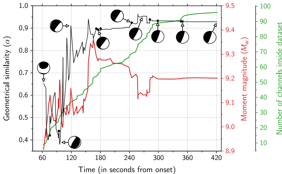
Figure 6. Same as Figure 5 but for \tau_c = h_d = 70 s. The color version of this figure is available only in the electronic edition.
