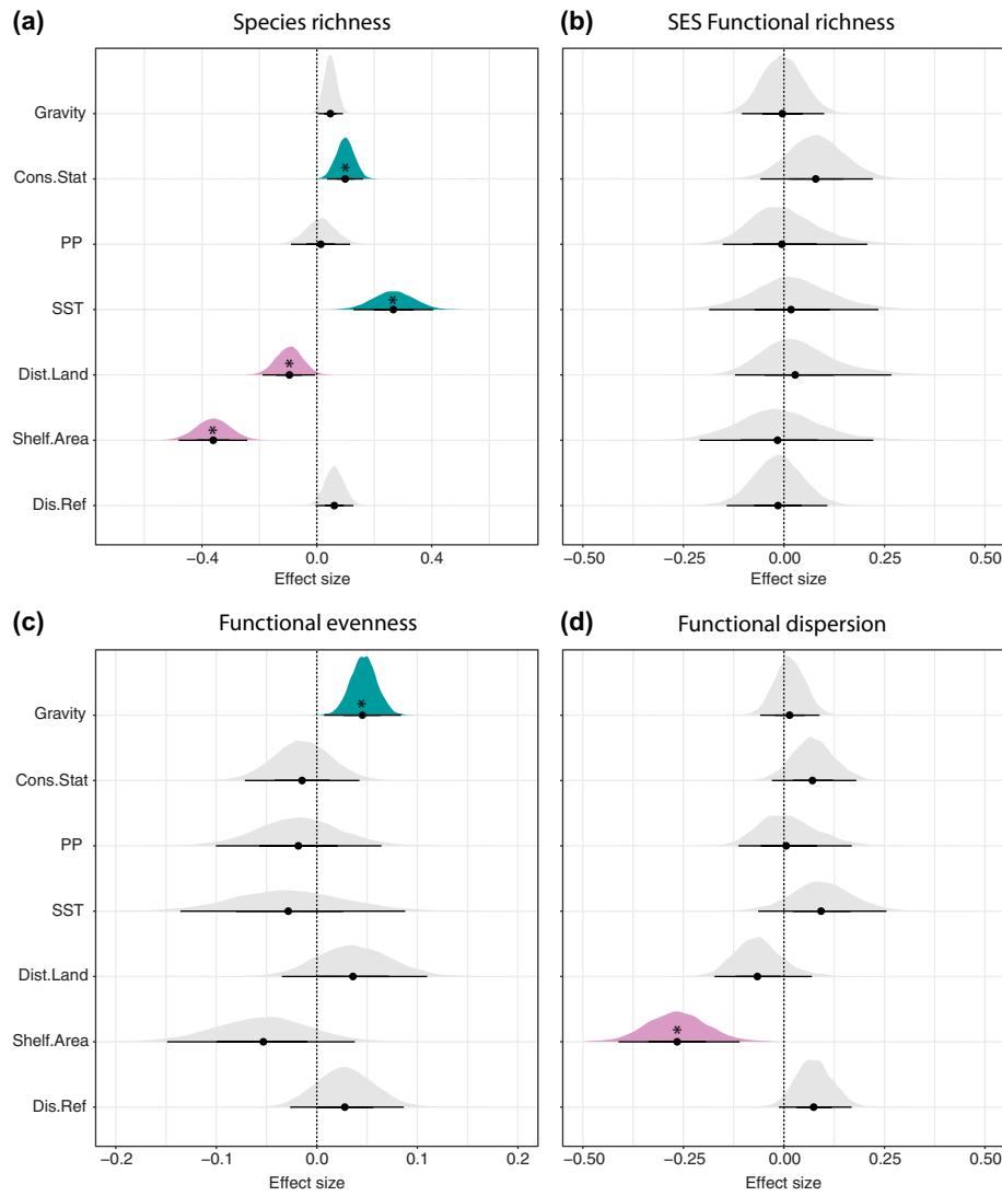
Figure 2. Effect of historical (Dis.Ref: distance from Quaternary refugia), biogeographic (Shelf.Area and Dist.Land: distance from the mainland), energetic (SST: sea surface temperature and PP: primary productivity), and anthropogenic (Con.Stat: Conservation status and Gravity: human population gravity) predictors on ETP reef fish diversity. Values are standardized as positive (blue) or negative (purple) effect sizes. Points represent mean parameter estimates, lines represent 95% credible intervals, and density plots represent the distribution of the effect sizes per factor. Asterisks denote factors that had a 95% credible interval of the posterior distribution not overlapping with zero.
