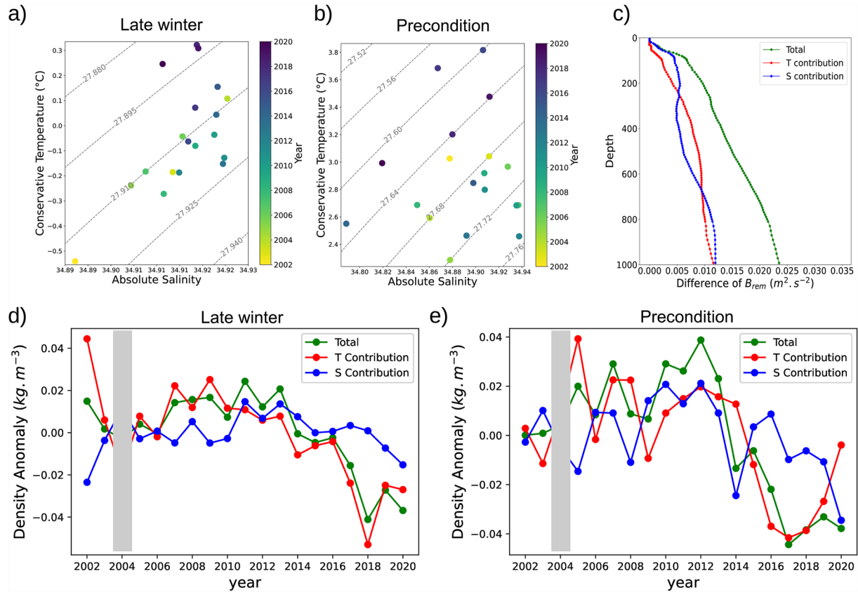
Figure 3. (a) Mean \Theta S-diagram within the mixed layer during the late winter and isopycnals as gray dotted lines (surface reference), with the years represented in colors. (b) Mean \Theta S-diagram above 500 m during the preconditioning period (September–December) and isopycnals (referenced to the surface) as gray dotted lines, with the years represented in colors. (c) Difference of buoyancy to be removed ( m^2 \cdot s^{-2} ) in the preconditioning period (September–December) between a non-convective (2014–2020) and a convective (2007–2013) periods. (d) Time series of the late winter density anomalies in the mixed layer. (e) Time series of the fall density anomalies in the top 500 m. For (c–e), the total is in green, and the salinity and temperature contributions are in blue and red, respectively.
