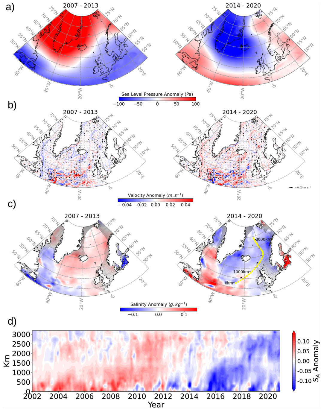
Figure 4. (a) Sea level pressure anomalies (in Pa) during the convective (left) and non-convective (right) periods. (b) Surface geostrophic velocity anomalies (in m \cdot s^{-1} ) provided by AVISO ( http://www.aviso.oceanobs.com ) during the convective (left) and non-convective (right) periods, the arrows are the mean velocity and direction for each period. (c) Absolute salinity anomalies (in g \cdot kg^{-1} ) in the top 300 m layer of the Nordic seas during the convective (left) and non-convective (right) periods, the hatched regions presented a percentage of variance higher than 75% and it is less trustworthy in these analyses. The anomalies are calculated in reference to the mean over the full period of analysis (2002–2020). (d) Time-distance plot of the monthly absolute salinity anomaly (in g \cdot kg^{-1} , referenced to the monthly mean over 2002–2020) averaged over 0–500 m in the path of the North Atlantic Current (yellow dots in panel c).
