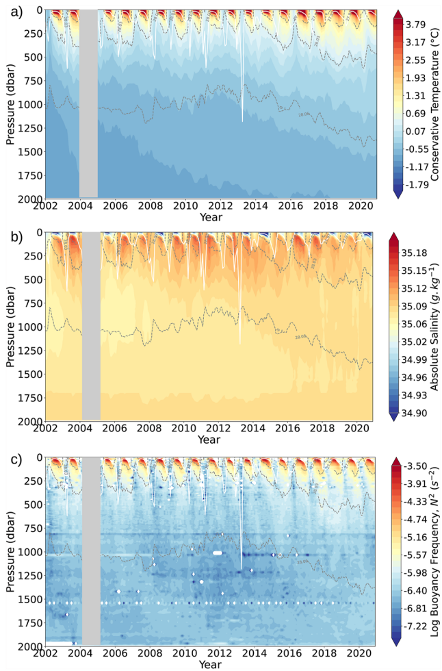
Figure 2. Time evolution of the profiles of (a) conservative temperature (in °C), (b) absolute salinity (in \text{g kg}^{-1} ), and (c) buoyancy frequency N^2 (shown in log scale, in \text{s}^{-2} ), averaged between 10^\circ\text{W} and 10^\circ\text{E} and 72^\circ\text{N} and 76.5^\circ\text{N} (red box on Figure 1a). The average mixed layer depth is shown as a white contour and isopycnals as a gray dotted contours (referenced to the surface). The year 2004 is masked as there is no observation during that winter.
