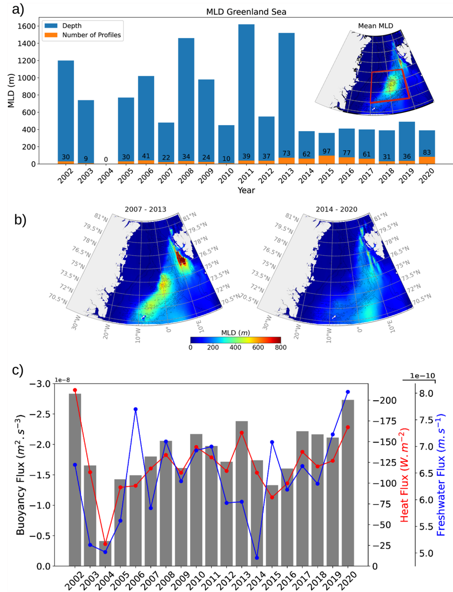
Figure 1. (a) Maximum mixed layer depth (MLD) (blue bars) per year in the Greenland Sea during late winter (February to April) in the red box area (between 10°W and 10°E and 72.5°N–76°N). The number of available Argo profiles in the box is shown in orange. The insert map shows the average (2002–2020) late winter MLD. (b) Maps of the mean MLD during the convective (left) and non-convective (right) periods. (c) Average air-sea flux in the center of the Greenland Sea (10°W to 10°E and 72°N to 76.5°N), during late winter (February–April). The total buoyancy surface flux (in m^2 \cdot s^{-3} ) is shown as Gray bars, and the heat (in W \cdot m^{-2} ) and freshwater flux (in m \cdot s^{-1} ) are shown as red and blue lines, respectively.
