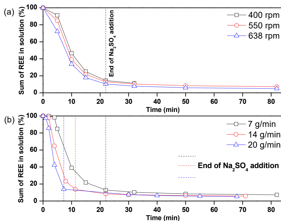
Figure 6. Influence of hydrodynamic parameters on the precipitation reaction of REEs (a) stirring rate ( T = 60\text{ }^{\circ}\text{C} ; Na:REE = 3.6:1; \text{Na}_2\text{SO}_4 = 7\text{ g/min} ) and (b) \text{Na}_2\text{SO}_4 flow rate ( T = 60\text{ }^{\circ}\text{C} ; Na:REE = 3.6:1; 550 rpm).
