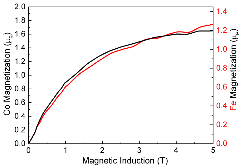
Figure 6: Field dependence of the maximum of XMCD signal at the L_3 edge for Fe (red line) and Co (black line). The XMCD intensity is converted into Bohr magnetons following the magnetic moment determination from Figure 5 (see text for more information).
