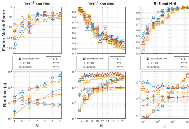
Fig. 2. Runtime and FMS [14] depending on 4 main complexity parameters N , T , R and I . Left plots: N experiment with N \in \llbracket 4, 10 \rrbracket . Middle plots: R experiment with R \in \llbracket 3, 20 \rrbracket . Right plots: experiment regarding T .
