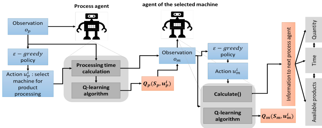
Fig. 2. The MARL model for the FFL scheduling problem.
