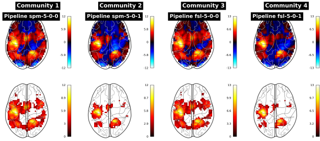
Fig. 3. Mean statistic map across groups of subjects for a representative pipeline of each community for the contrast right-hand . Unthresholded (upper) and thresholded maps (lower) with FDR-corrected p < 0.05 .
