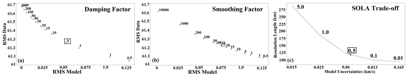
Figure 7 Trade-off curves (L-curves) for Fast-marching (a,b) and SOLA inversions (c). A trade-off between data residual and model variance for different values of the damping (a) and smoothing (b) parameters for the Fast-marching Surface-wave Tomography method. (c) A trade-off between average resolution and average uncertainty for the SOLA method for different values of the trade-off parameter \eta . The numbers in the boxes show the chosen trade-off value for the period of 10s.
