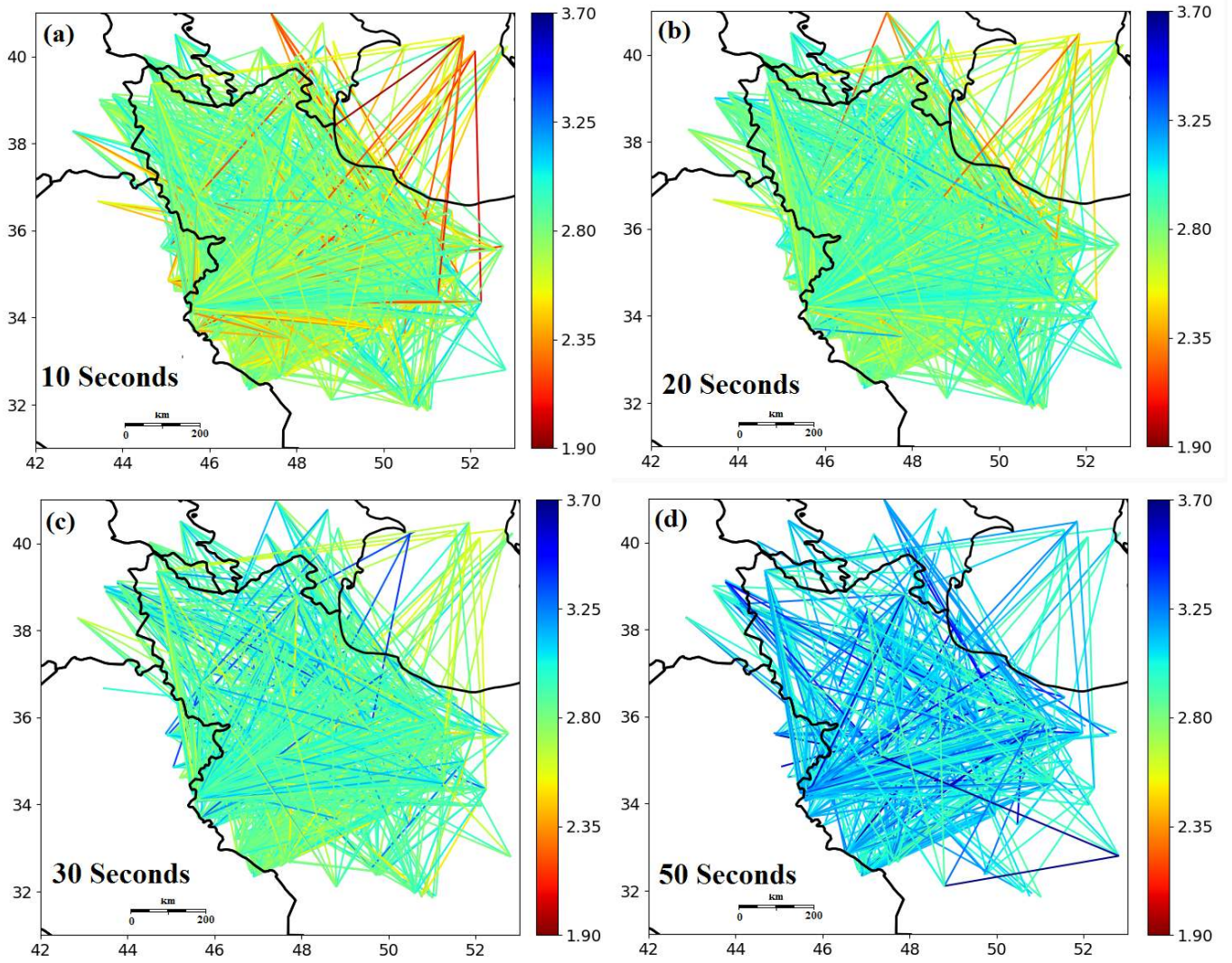
Figure 6 Path coverage of group-velocity measurements at periods of 10, 20, 30, and 50 s. Paths are colored by their respective group-velocity values.
