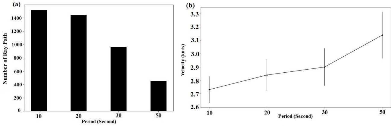
Figure 5 (a) The number of group-velocity measurements at periods of 10, 20, 30, and 50 s. (b) The average group-velocities at each period; the error bars show the average uncertainties of the measurements at each period.
