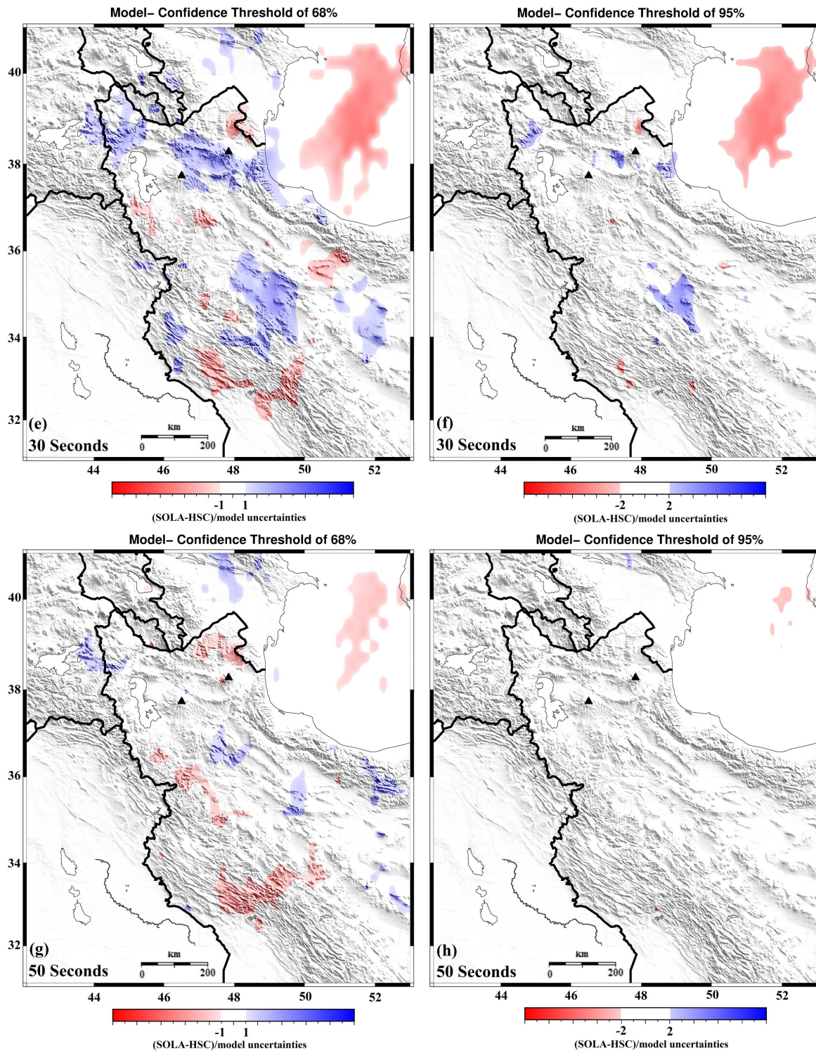
Figure 16 Group-velocity anomalies scaled by the SOLA uncertainties \sigma_m at periods of 30, and 50 s. (e) and (g) are masked at \pm 1\sigma_m ; (f) and (h) are masked at \pm 2\sigma_m . We masked all cells with fewer than three rays passing through them.
