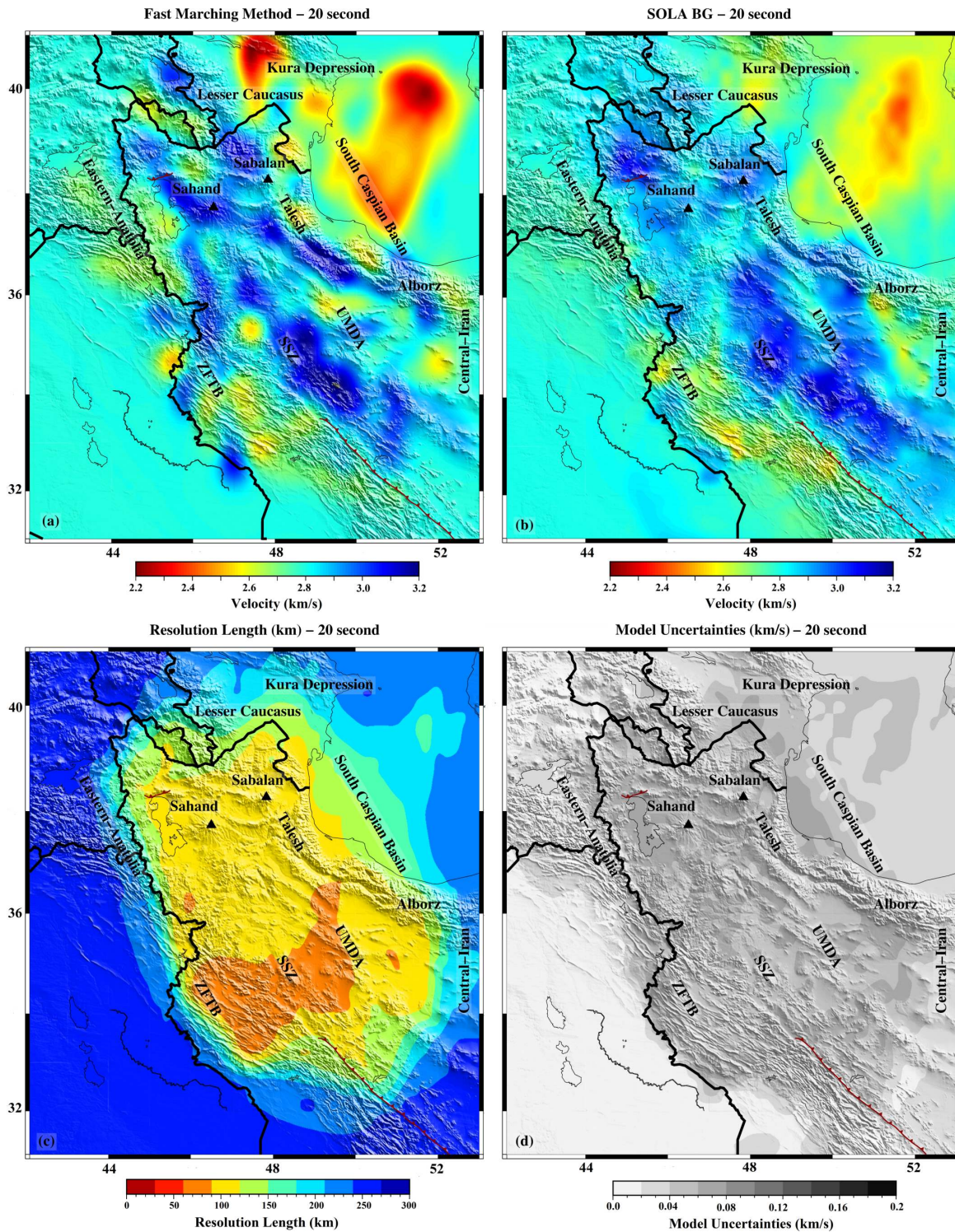
Figure 12 Tomographic results for group velocities at 20 s period. Panels as in Fig. 11.
