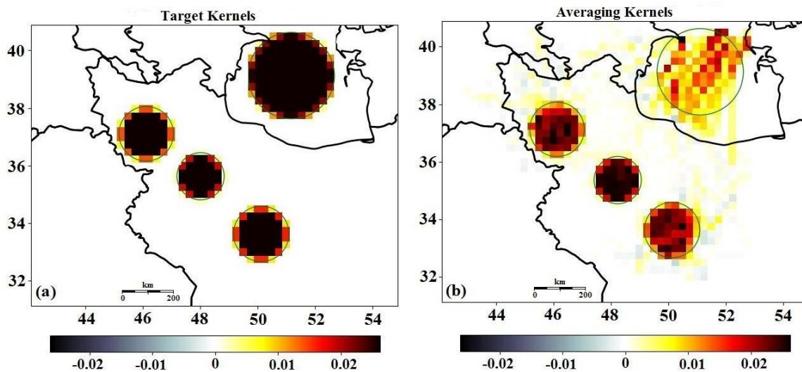
Figure 9 Target and averaging kernels for the SOLA inversion at 10 s period. (a) Circular target kernels at locations with different path densities. (b) Averaging kernels obtained after a SOLA inversion with \eta = 0.4 .
