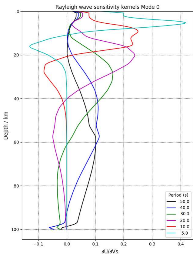
Figure 10 Sensitivity kernels of Rayleigh-wave group velocity at different periods.
