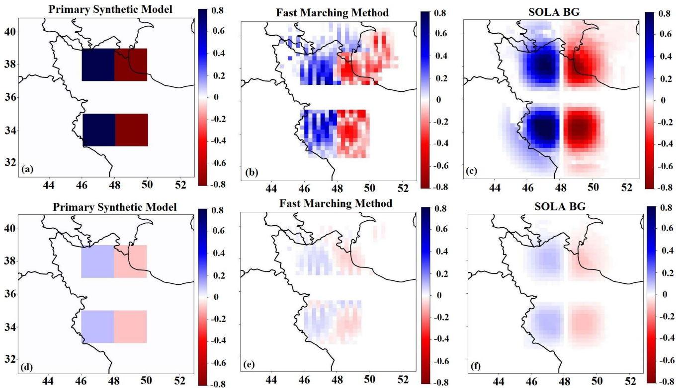
Figure 17 Synthetic tests for different regions. (a) and (d) are unfiltered synthetic model with sharp and weak anomaly contrasts, respectively. (b) and (e) are filtered models with Fast-marching method. (c) and (f) are filtered model with SOLA Backus-Gilbert. The ray-coverage used corresponds to the 20 s coverage from Fig. 6.
