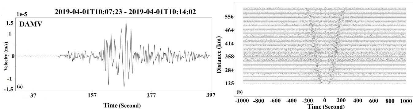
Figure 2 (a) Example of the vertical component of a seismogram (in velocity) used for dispersion measurements, filtered between 5 s and 120 s. Horizontal axes show time duration after origin time. The signal is detrended, decimated and station responses have been removed. Station names and times are shown. (b) Vertical two-sided noise correlation functions sorted by inter-station distance. The surface-wave move-out is between 2 and 4 km/s. Rayleigh-waves are observable at both positive (causal) and negative (acausal) lag times. Only the noise correlation functions with signal-to-noise ratios larger than 10 are plotted.
