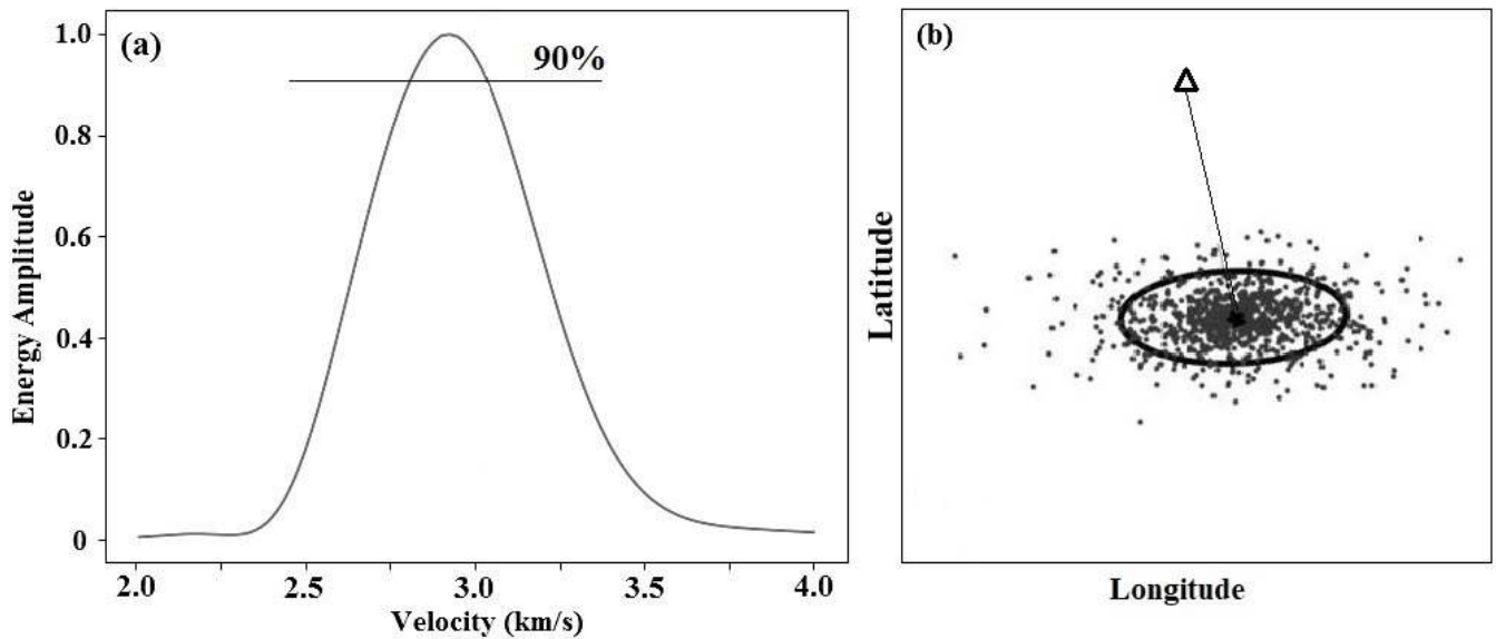
Figure 4 (a) From the dispersion diagrams in Fig. 3, we extract plots of energy versus velocity at a given period (in this example 50 s). We estimate the uncertainty of the velocity measurement from the range of velocities at which the seismic energy is at least 90% of that at the apex of the curve. (b) Schematic figure of the data error related to the location of the earthquake. The error ellipse is drawn around the exact location of the events and uniform points with Gaussian distribution surrounding it.
