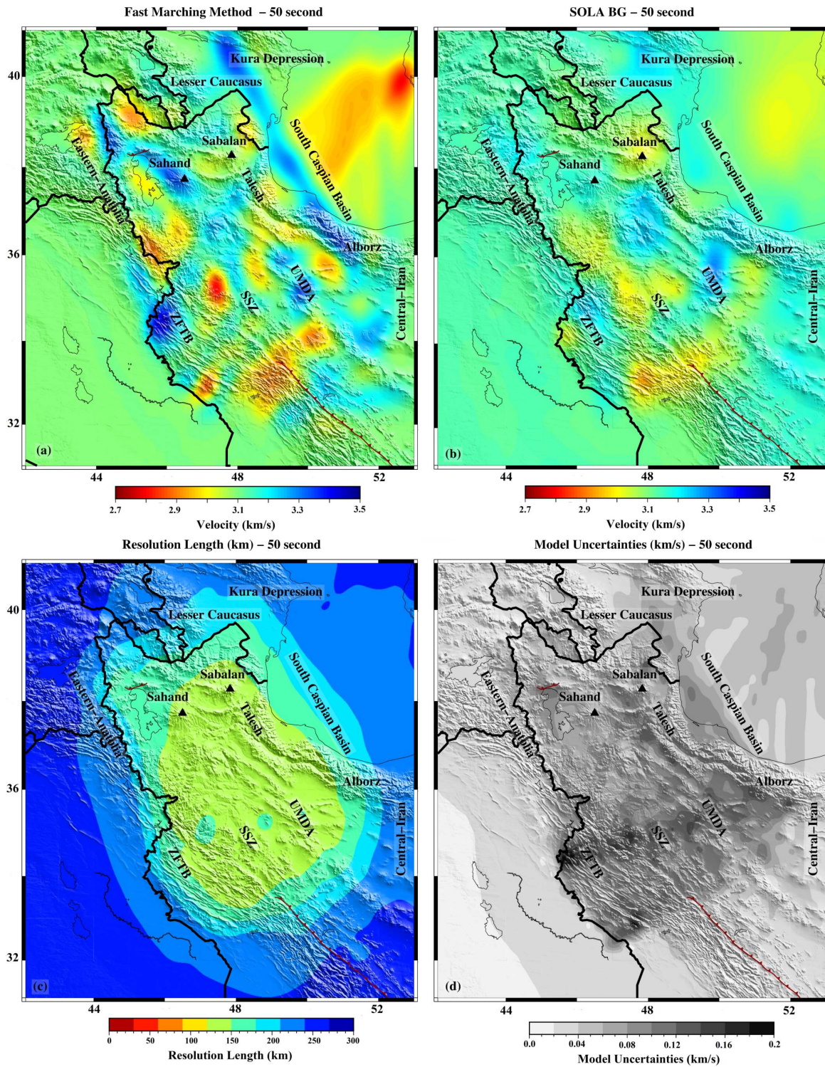
Figure 14 Tomographic results for group velocities at 50 s period. Panels as in Fig. 11.
