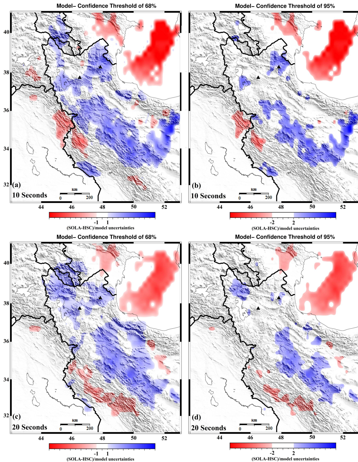
Figure 15 Group-velocity anomalies scaled by the SOLA uncertainties \sigma_m at periods of 10 and 20 s. (a), (c), are masked at \pm 1\sigma_m ; (b), (d), are masked at \pm 2\sigma_m . We masked all cells with fewer than three rays passing through them.
