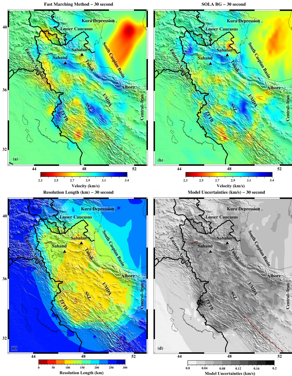
Figure 13 Tomographic results for group velocities at 30 s period. Panels as in Fig. 11.
