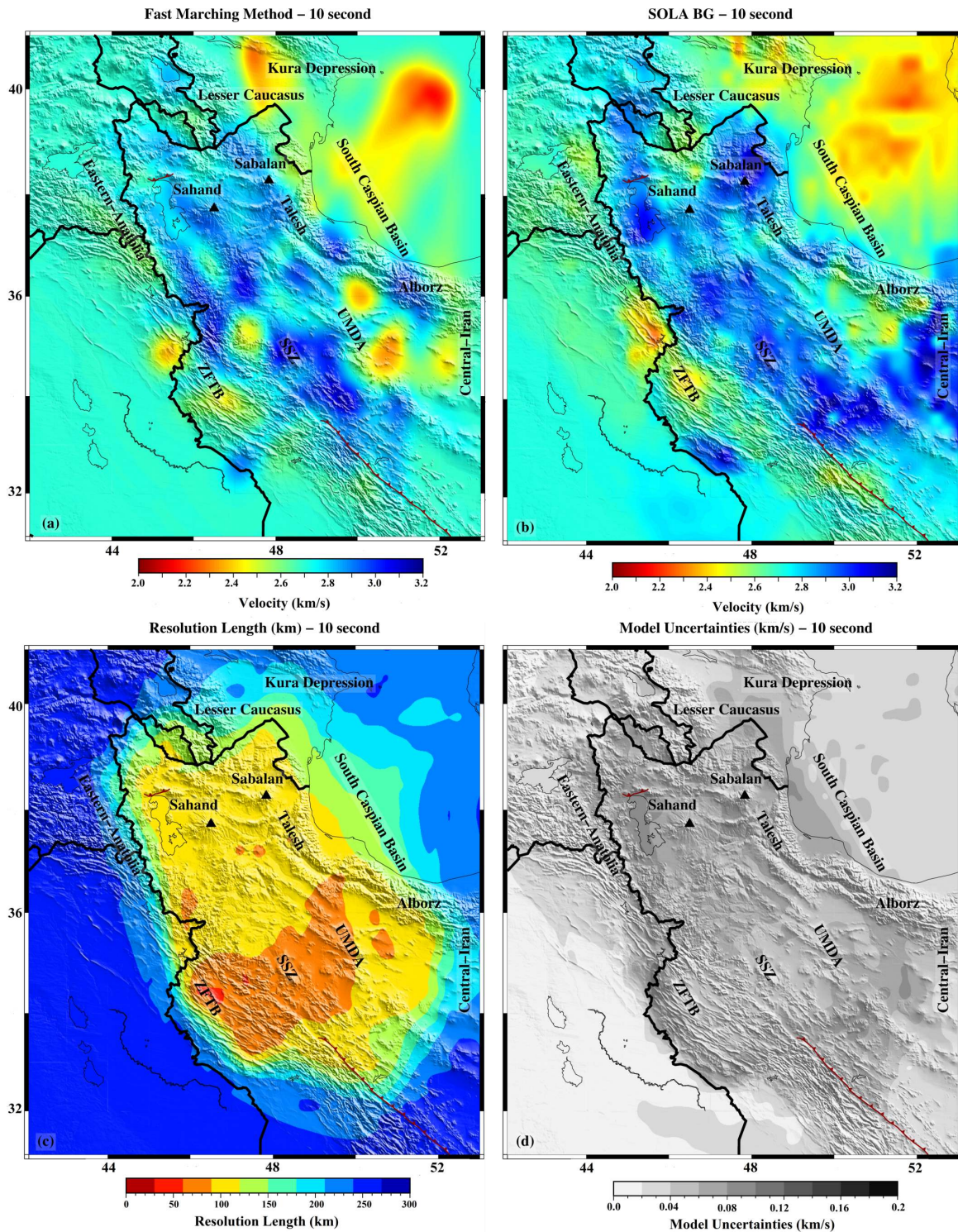
Figure 11 Tomographic results for group velocities at 10 s period. (a) Group velocity map obtained using Fast-marching tomography. (b) Group velocity map obtained using SOLA Backus-Gilbert tomography. (c) Resolution lengths and (d) model variances from the SOLA inversion.
