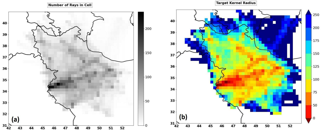
Figure 8 Path densities and SOLA target kernel radii at 10 s period. (a) The number of paths per 0.25^\circ cell. (b) Radii of target kernels derived from the path densities using equation 6; cells containing no paths are masked in white.
