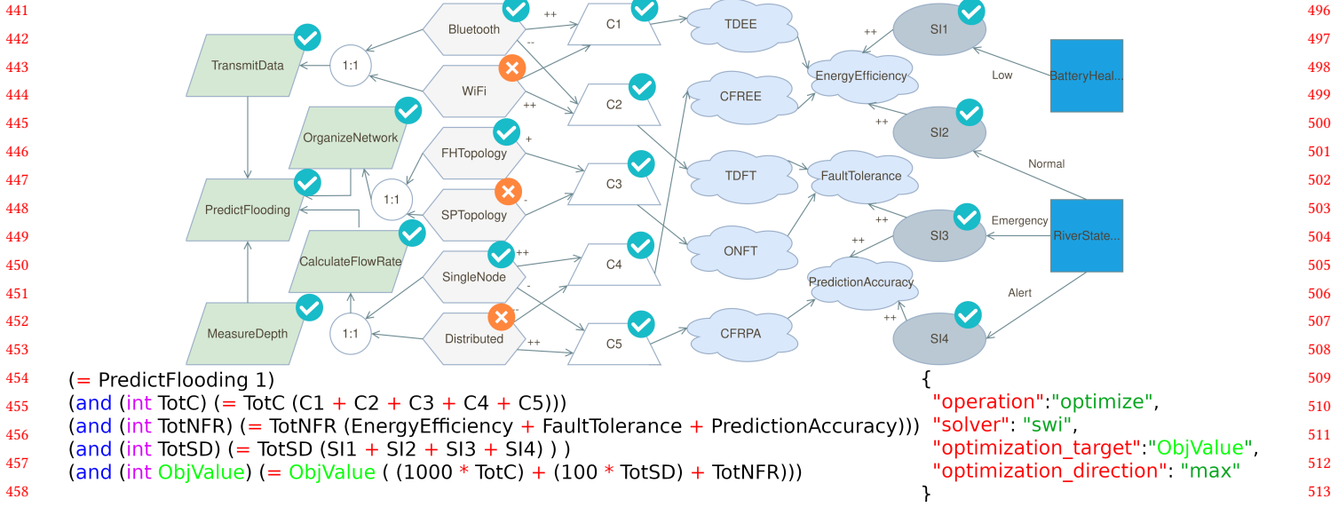
Figure 2. Second part of our running example with a model using Sawyer et al.’s DSPL VML. This model reproduces the original example from the paper [40] for a flood early-warning system. As with our other example, in addition to a reasoning query to solve (on the bottom right), this time, an optimization problem to find an optimal configuration whose additional constraints are shown below the model (bottom left).
