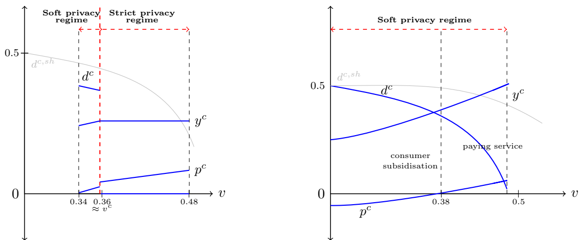
Figure 5: Left : \sigma = 1 , \alpha = \underline{0.25} , t = 0.06 ; Right : \sigma = 1 , \alpha = \underline{0.5} , t = 0.06 .
