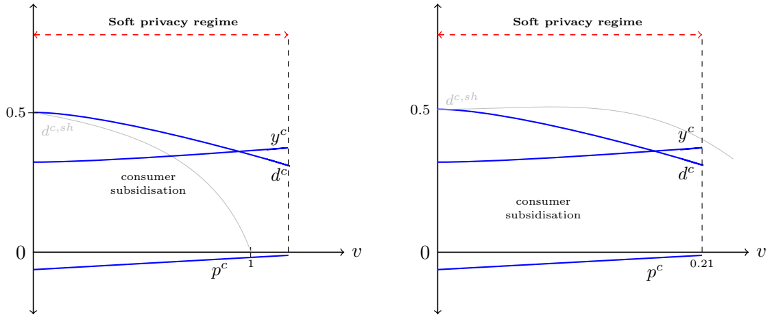
Figure 4: Left : \sigma = \underline{0.2} , \alpha = 0.5 , t = 0.04 ; Right : \sigma = \underline{1} , \alpha = 0.5 , t = 0.04 .
