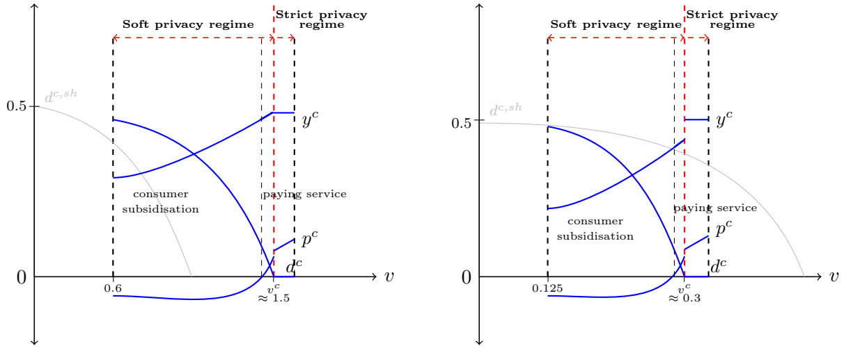
Figure 3: Left : \sigma = \underline{0.2} , \alpha = 0.25 , t = 0.04 ; Right : \sigma = \underline{1} , \alpha = 0.25 , t = 0.04 .
