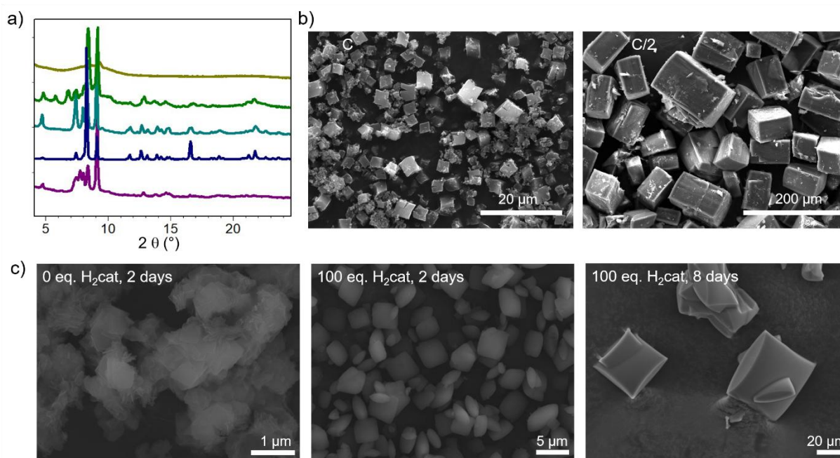
Fig. 3 a) PXRD patterns of the samples synthesized in various solvents; from top to down: pure DEF, DEF/ H_2O = 3, DEF/ H_2O = 1, DEF/ H_2O = 1 and concentration lowered twice, DEF/ H_2O = 1/3; b) SEM images of CatPMOF-2(Al): effect of the concentration of reactants; c) SEM images
