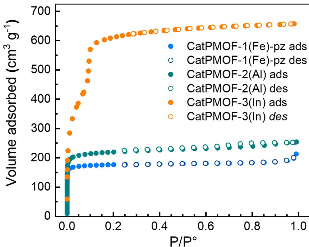
Fig. 10 Nitrogen sorption isotherms measured at 77 K, evidencing that all phases are porous.
