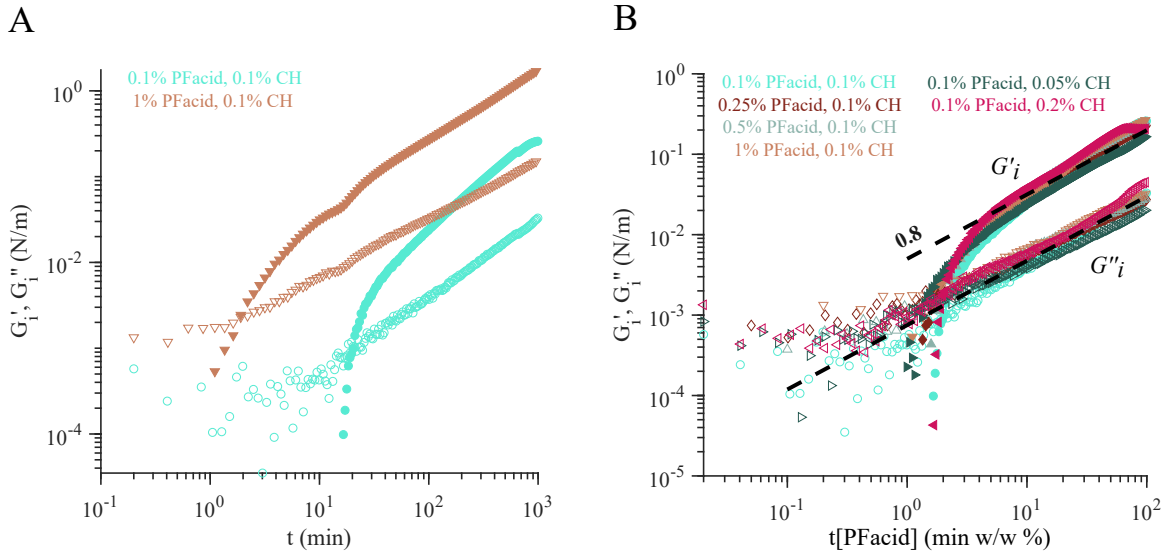
Figure 3: Macroscopic study of the interfacial rheological properties of a chitosan / PFacid membrane. (A) Typical time-dependent evolution of interfacial elastic G'_i (filled symbols) and viscous G''_i (empty symbols) shear moduli at different concentrations of PFacid. f = 0.5 Hz, \dot{\gamma} = 0.03\% , chitosan 0.1% w/w (B) The kinetics of G'_i and G''_i collapsed on the same master curves when the time axis was multiplied by the concentration of PFacid, for various concentrations of PFacid and chitosan.
