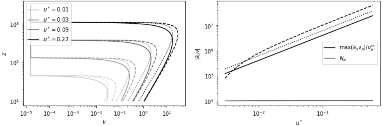
Figure 2: Left panel: O'Brien KPP viscosity profile \nu_a^{\text{O'Brien}} given by (9) (plain line), \nu_{1,a} (dashed line) and \nu_{2,a} (dotted line) given by definition 4.3 for different values of u^* . Right panel: the corresponding values of \|\partial_u \nu\|_{L^\infty(\Omega_a)} / \nu_a^m (black lines) and N_a(u^*) = \|\partial_u \nu(u^*) / \nu(u^*)\|_{L^\infty(\Omega_a)} (grey line) for \nu_a^{\text{O'Brien}} only.
