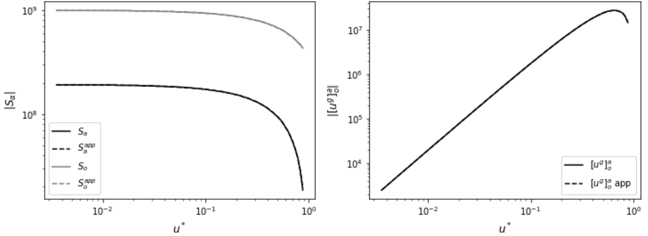
Figure 1: Left panel: computed S_\alpha (plain lines) for O'Brien KPP viscosity profile (definition (2.2)) and their approximations given by (44) (dashed lines). Curves are superimposed. Right panel: corresponding profile of |\phi^g|_o^a| = |F(u^*)|
