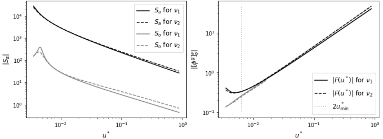
Figure 3: For KPP viscosity profiles with reference values (see definitions 2.2). Left panel: \mathcal{S}_\alpha given for, \nu_{\alpha,1} in continuous line, \nu_{\alpha,2} in dashed line. Black lines correspond to the atmospheric part and grey lines to the oceanic part. Right panel: the corresponding profiles of |\llbracket \phi^g \rrbracket_o^a| = |F(u^*)| with the same line style. Dot-dashed line and dotted line are superimposed. Black lines correspond to the case of fixed \delta_\alpha and grey lines to the case \delta_\alpha = h_\alpha/4 .
