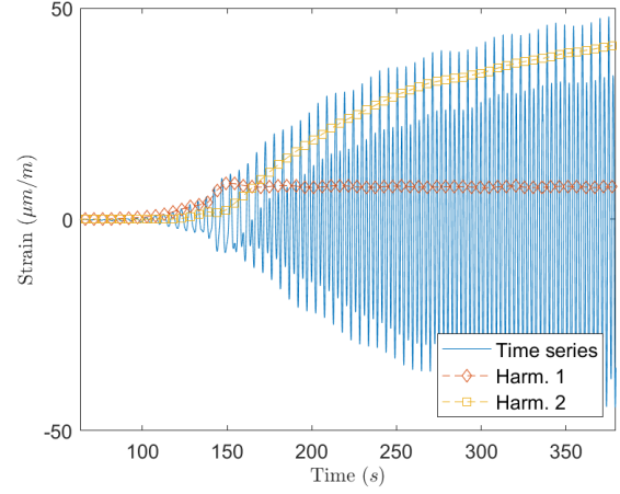
Figure 12: Bending strain ( e_2 ) time series (including transient) at T = 5.2 s and with \frac{H}{\lambda} = 6 %.
