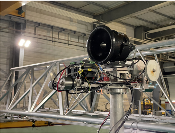
Figure 3: Photo of the RNA. The thruster is visible in black. Masses are added to adjust the position of the COG.
