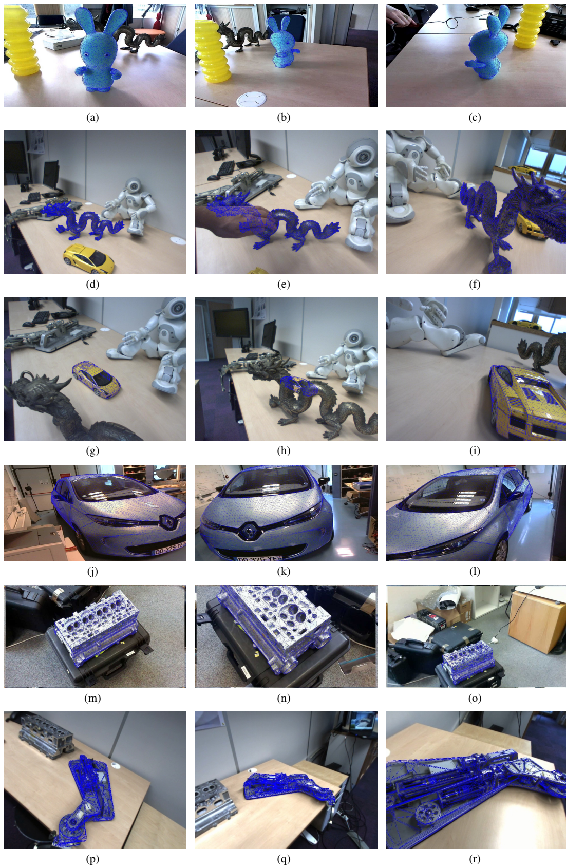
Fig. 24: Accurate localization results on a Raving Rabbid, a dragon, a sport car, a real-sized car, a car cylinder head, and an orthosis with our phDEC-SLAM. Results are similar with rDEC-SLAM and rhDEC-SLAM. The accuracy can be appreciated by the projection of the 3D blue models on the object of interest in the images.
