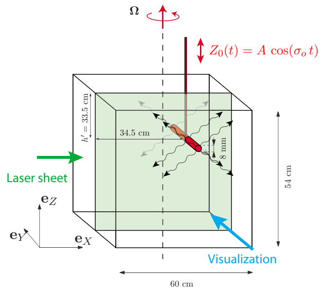
FIG. 2. (Color online) Schematic view of the experimental setup. The horizontal 8 mm diameter cylinder is oscillating vertically according to Z_0(t) = A \cos(\sigma_o t) , with A=2 mm and \sigma_o=0.2 Hz. PIV measurements in a vertical plane ( X, Z ) in the rotating frame are achieved by a vertical laser sheet and a camera at 90°.
