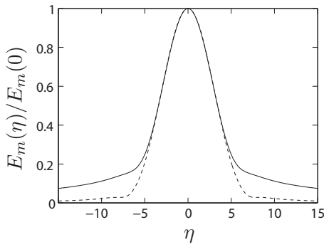
FIG. 14. Normalized velocity [(-) m=0 ] and vorticity [(- -) m=1 ] envelopes of the similarity solutions.
