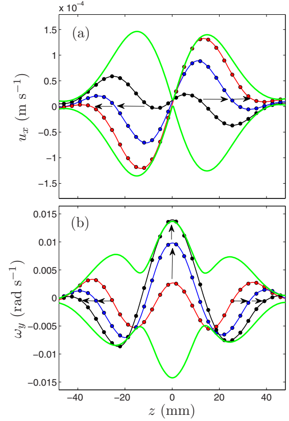
FIG. 10. (Color online) (a) Velocity envelope u_0(x_0, z) and three velocity profiles u_x(x_0, z, \phi) as a function of the transverse coordinate z at a fixed distance x_0 = 70 mm (average over 50 < x < 90 mm) from the wavemaker for \sigma_o/2\Omega = 1 . (b) Corresponding vorticity envelope and vorticity profiles. The arrows indicate the time evolution of the profiles. The interference of the upward and downward wave beams produces a stationary wave pattern at z=0 with a velocity node and a vorticity maximum. Same data representations as in Fig. 9.
