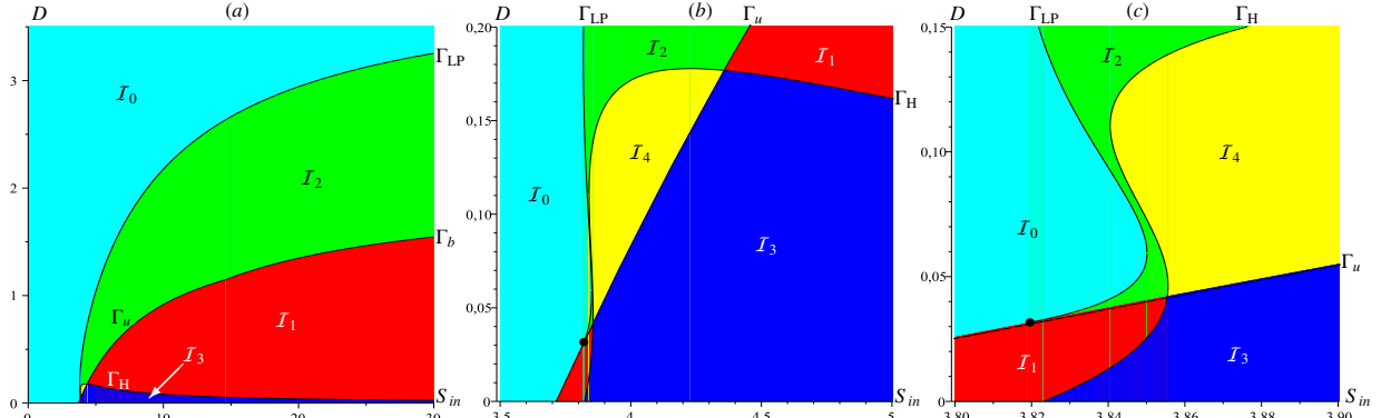
Figure 2: Operating diagram of (1). (a) The case considered in Section 3.3. (b-c) Magnifications of (a) showing the curve \Gamma_H .
