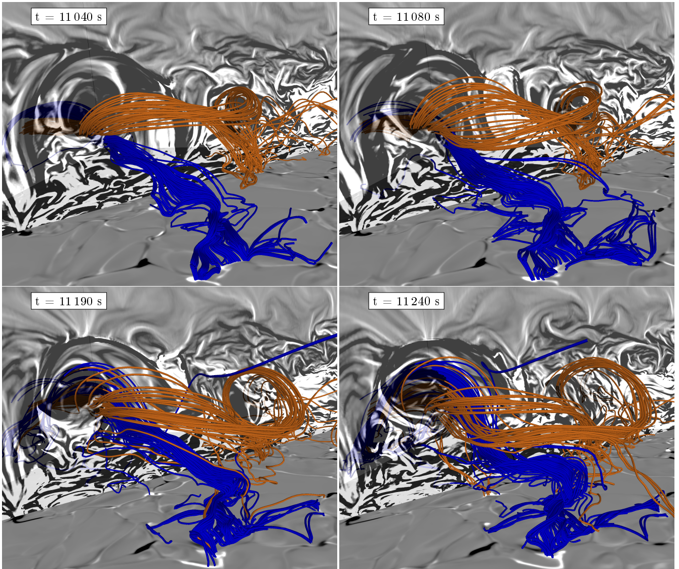
Fig. 4. Zoomed-in 3D renderings of the flux bundles associated with the contours shown in the center and lower panels of Fig. 3.
