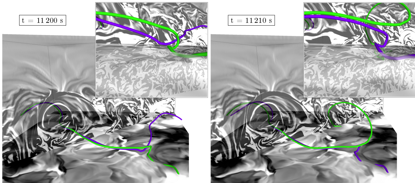
Fig. 6. Field line pair at t = 11\,200 s (left) and t = 11\,210 s (right) that are traced by the same two Lagrangian markers, but switch chromospheric footpoints between the two time stamps. The insets in the upper right corners offer a zoomed-in view of the footpoint switching at a different viewing angle, as evidenced by the lines switching colors.
