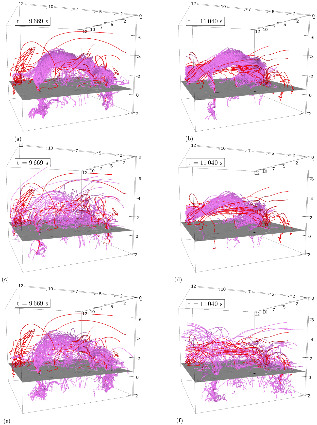
Fig. A.1. Upper panels illustrate a horizontal flux system seeded consistently in space at t = 9669 s (left) and t = 11040 s (right). Red lines are seeded with Lagrangian markers as reported in Robinson et al. (2022). Center panels illustrate the time evolution of a horizontal flux system seeded by Lagrangian markers at t = 11040 s (right) and traced backward in time (left). Lower panels are the same as center panels, except seeded by Lagrangian markers beginning at t = 9669 s (left) and traced forward in time (right).
