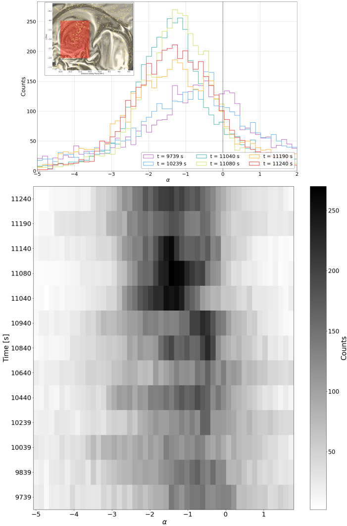
Fig. 7. Time series of \alpha histograms corresponding to the same time stamps as in Fig. 3 (upper). The inset in the upper left corner shows the area within the flux rope center where these statistics were calculated. The lower panel shows a 2D histogram time series for several time stamps ranging from t = 9739 s until 11 240 s.
