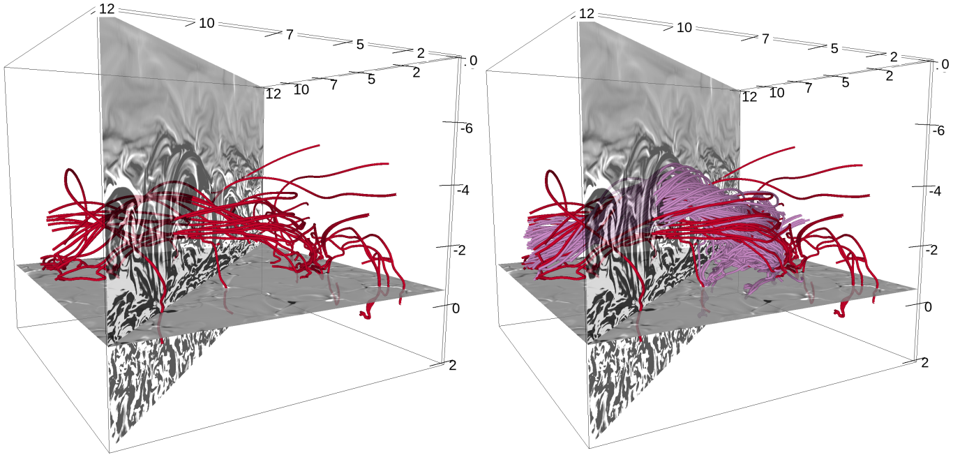
Fig. 1. Magnetic field lines at t = 11\,040 s belonging to a flux rope as analyzed in Robinson et al. (2022), with a bisecting plane colored by saturated \alpha values (left). The right panel is the same as left panel, with the addition of lines corresponding to the wider flux rope that was first seeded by its proximity to the thin current sheets in the rope near the orthogonal slice, then seeded by corks that were geometrically closest to those lines at that time.
