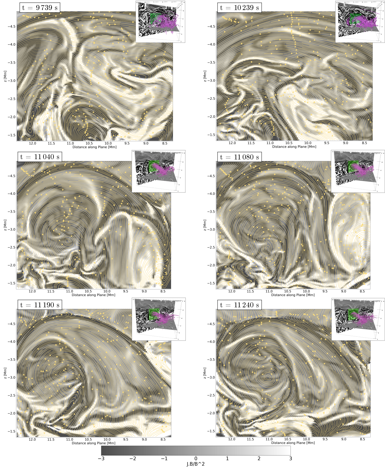
Fig. 3. Vertical slices showing \alpha (Eq. (1)) along an orthogonal plane with respect to the flux rope. Yellow contours represent the field strength along the plane with arrows indicating the direction of twist. Each panel represents a different timestep, and each includes a 3D inset showing the vertical plane colored by \alpha and showing flux rope lines. The green box on the inset represents the size and location of the contour plot.
