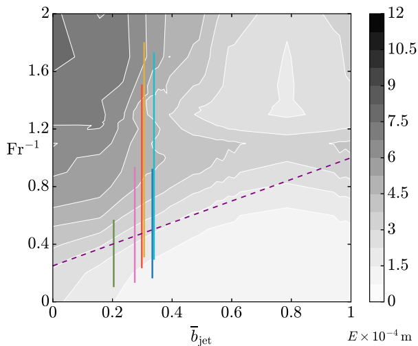
Fig. 7. Total extinction E for RH = 140\% . For the color line legend, see fig. 6
