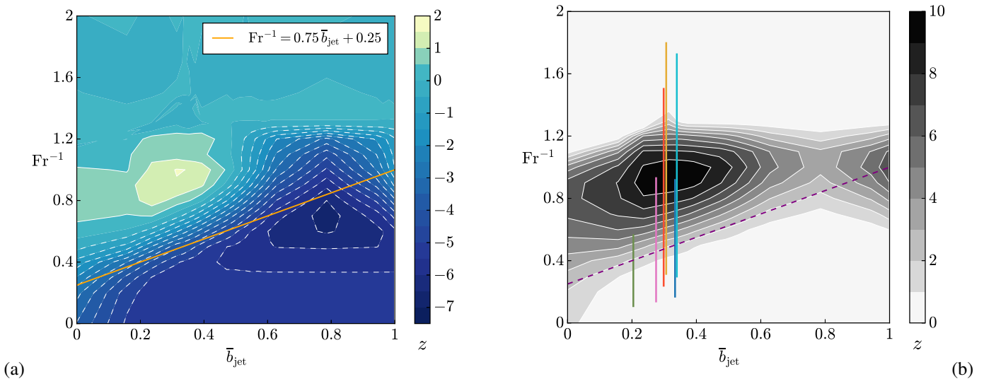
Fig. 6. (a) Mean altitude of the plume and (b) difference between the mean altitude of the plume and that of the vortices at t = 5\tau_0 as a function of Fr^{-1} and \bar{b}_{jet} . The vertical lines represent the range of possible parameters for a selection of twin-engine aircraft (from left to right): CRJ, B737, B777, A330, A320, B787. The purple dashed line on the right panel corresponds to the orange line on the left panel.
