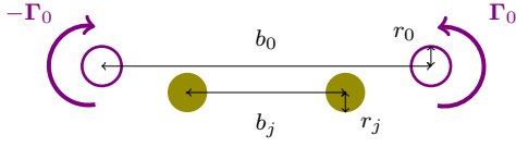
Fig. 1. Setup of the initial flow.
