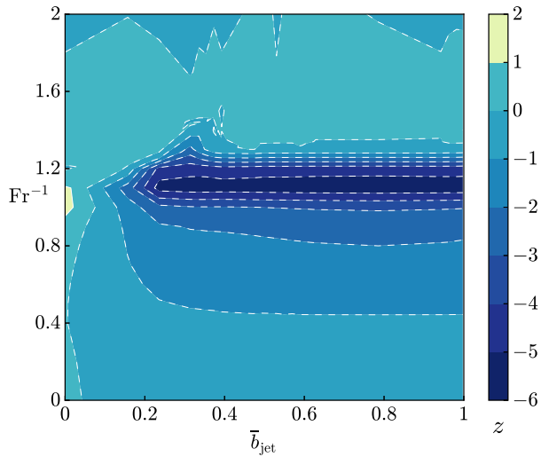
Fig. 4. Altitude modification of the vortex dipole due to hot jets as a function of Fr^{-1} and \bar{b}_{jet} .
