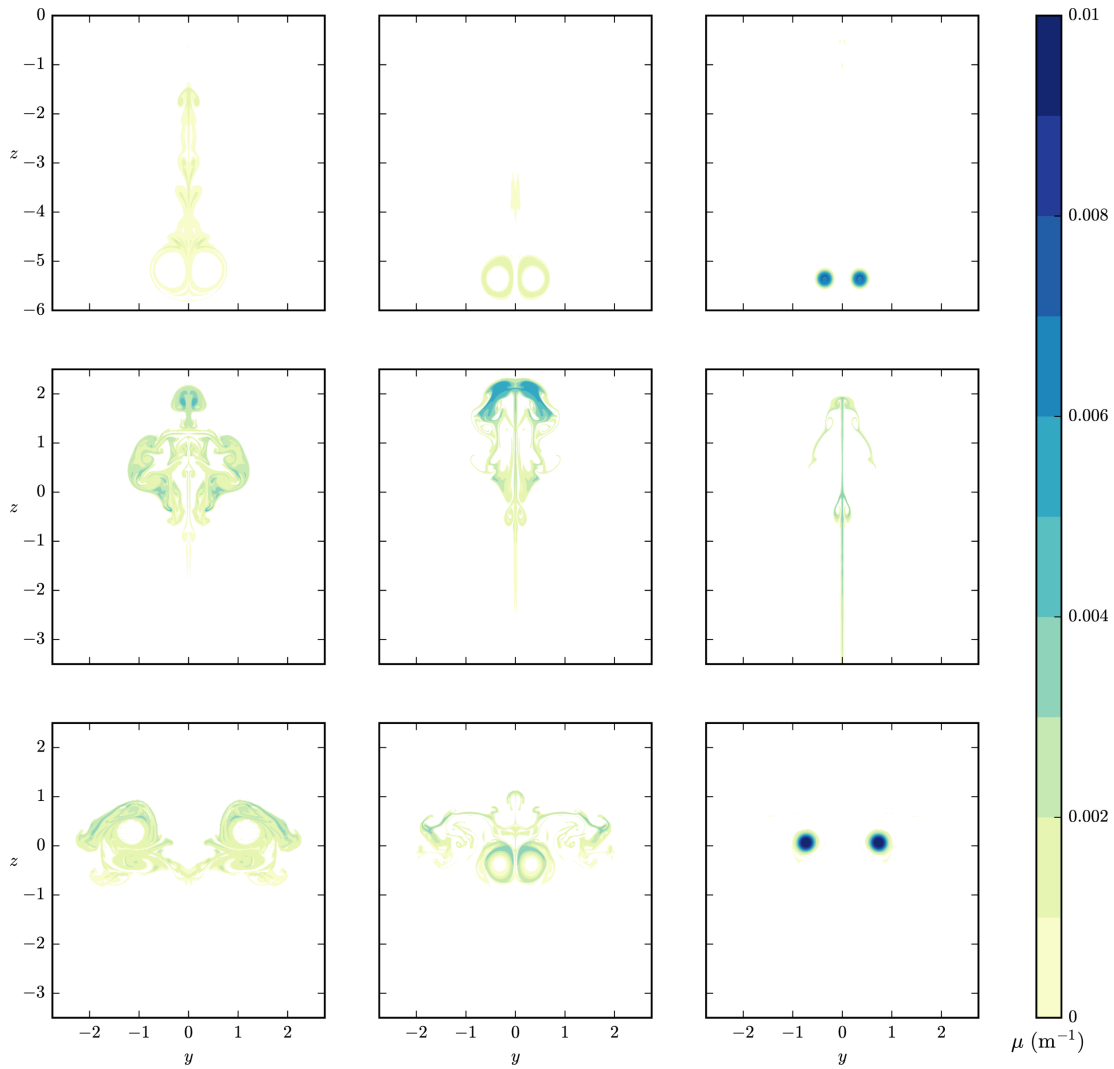
Fig. 8. Attenuation coefficient \mu at t = 5\tau_0 for RH_i = 130\% . From left to right \bar{b}_{jet} = 0.16, 0.31 and 0.79 . From top to bottom Fr^{-1} = 0.2, 1 and 1.4
