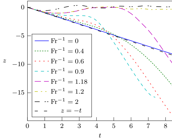
Fig. 2. Altitude of the vortices as a function of time for different values of Fr^{-1} . Distances are normalized by b_0 and time by \tau_0 .
