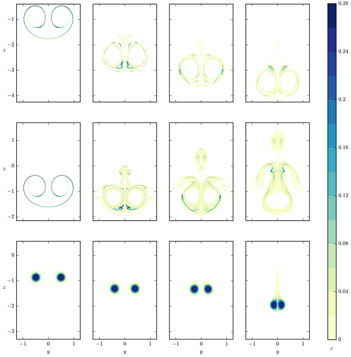
Fig. 5. Evolution of the passive scalar field over time. From top to bottom: \text{Fr}^{-1} = 0.2 , \bar{b}_{\text{jet}} = 0.16 ; \text{Fr}^{-1} = 1 , \bar{b}_{\text{jet}} = 0.16 ; \text{Fr}^{-1} = 1 , \bar{b}_{\text{jet}} = 0.79 . From left to right: t = \tau_0 , 2.5 \tau_0 , 3 \tau_0 , 3.5 \tau_0 .
