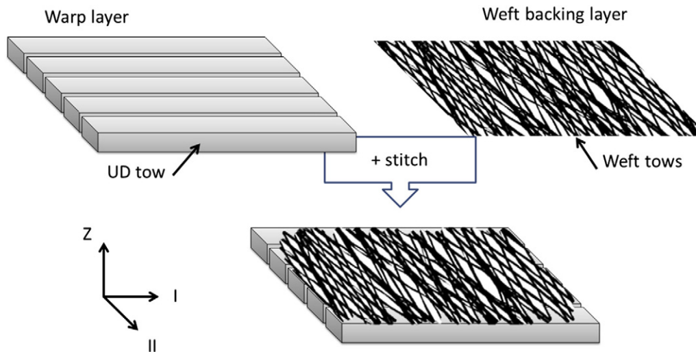
Fig. 17. 3D representation of quasi-UD NCF fabric [28].
