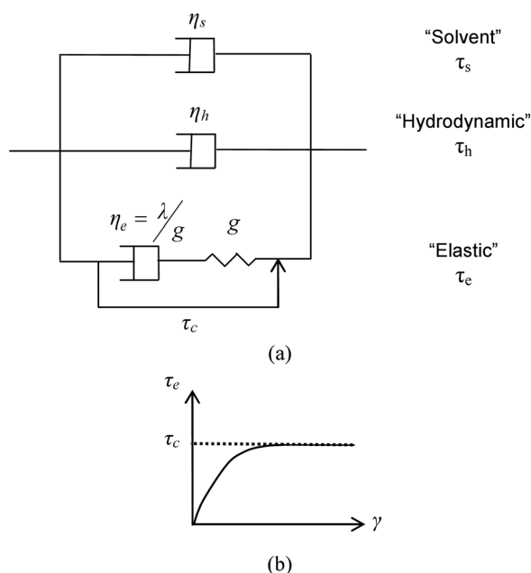
FIG. 10. (a) The mechanical analogue for the CB and CNT suspensions, termed the “structure-dependent hybrid Maxwell-Voigt phenomenological model with yield stress”; (b) the effect of the slider is to limit the maximum stress an element can support at large strains.
