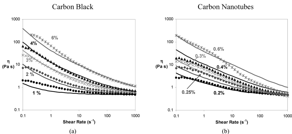
FIG. 11. Model fit (solid line) to the experimental apparent viscosity data (points) as a function of shear rate for (a) CB dispersions and (b) CNT suspensions. The model parameters were as shown in Table III.
