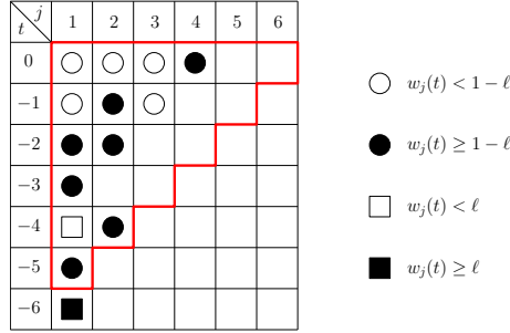
Figure 10: Illustration of the execution of Algorithm 1 on an example, in the case where \ell < 1 - \ell . The variables sampled until the Boolean variable Stopping becomes True are pictured by black/white squares and disks. One searches for the first time T^* such that every line of index T^* + 1 \leq t \leq 0 has at least one black disk between columns 1 and t - T^* and such that there is a black square in position (T^*, 1) . The full triangular array of variables used in the construction of \nu is enclosed by a red boundary.
