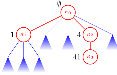
Figure 7: A possible evolution of the PWIT with the vertices of \mathbb{K} embedded correctly. The little triangle at the end of blue particles symbolize the blue descendants produced by each blue particle, which play no role in the coupling, hence do not interact with \Phi or the times at which the red particles appear. However, the blue particles represented here play a role, as they influence the label given to each of the red particle.
