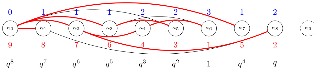
Figure 6: The first 9 vertices of C are shown, together with the edges between them. Vertices of G not connected to 1 via a path are not shown. The number above each vertex \kappa_j is the maximal path length L_{\kappa_j} . The number below each vertex is its rank. The thick edges are the edges of the special spanning tree B . To explain this, consider, e.g., vertex \kappa_6 and observe that it is connected to \kappa_4 with L_{\kappa_4} = 2 and to \kappa_3 with L_{\kappa_3} = 1 ; so we choose \kappa_4 as the parent of \kappa_6 in B . Consider vertex \kappa_8 . It is connected to vertices \kappa_2 and \kappa_1 with L_{\kappa_2} = L_{\kappa_1} = 2 . Since \kappa_2 has lower rank than \kappa_1 we declare that \kappa_2 is the parent of \kappa_8 in B . Finally, the quantities on the lower line are proportional to the probability that \kappa_9 chooses its parent among the existing vertices, i.e it will be connected to e.g. \kappa_8 with probability \frac{q}{1+q+q^2+q^3+q^4+q^5+q^6+q^7+q^8} .
