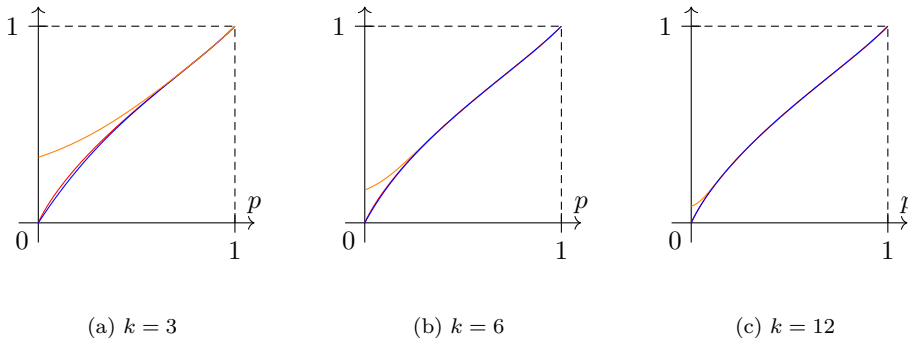
Figure 5: Successive bounds on the function C (in red) by \overline{C}_k (in orange) and \underline{C}_k (in blue). Observe that if these bounds appear very sharp for p close to 1, the approximation (in particular the upper bound) remains quite crude for p close to 0.
