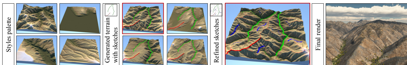
Figure 1: Our diffusion-based terrain authoring framework empowers users to iteratively combine terrain stylization with feature sketching. Here, an artist first sketches a simple ridge and forked drainage network, then makes their style selection (outlined in red) before adding further details.
