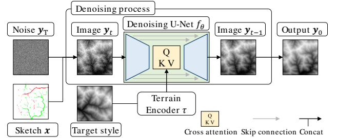
Figure 6: Our diffusion model architecture supports stylization using a terrain encoder and cross-attention, and feature sketching through concatenation with the input noise image. The denoising process applies a U-Net to iteratively reduce noise and introduce structure.
