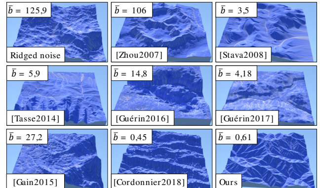
Figure 8: A comparison of drainage areas for different synthetic terrains: our method produces fewer endorheic pits and greater hydrological consistency (as measured by average breaching volume \bar{b} ) than previous data-driven approaches. Instances of procedural (ridged noise) and simulation [CCB*18] outputs are included for a basis of comparison. A lower breaching volume, \bar{b} , is better.
