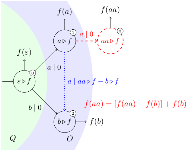
Fig. 5: Example of a partial execution of Algorithm 1 to build a k -residual transducer of a function f: A^* \rightarrow \mathbb{Z} such that aa \triangleright f \sim_k b \triangleright f . Nodes are labelled by their creation time. At this stage, Q = \{\varepsilon \triangleright f\} , O = \{a \triangleright f, b \triangleright f\} . The red node is not created, and the blue transition is added instead, corresponding to the “else” branch line 10 of Algorithm 1.
