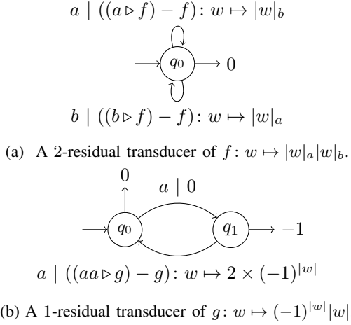
Fig. 4: Two residual transducers.
