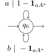
(b) A \mathbb{Z}\text{Poly}_0 -transducer computing \mathbf{1}_{aA^*} .
