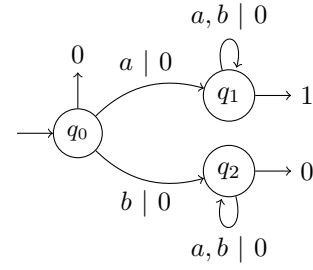
(a) A \mathbb{Z}\text{Poly}_{-1} -transducer computing \mathbf{1}_{aA^*} .
