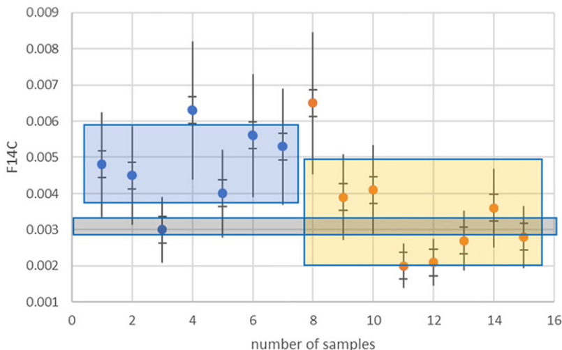
Figure 2 F 14 C results of the 15 bone blanks to test leaching of carbon from the XAD resin. Each point has a small error bar representing only the counting statistics and C 13 H correction, and a larger error bar representing the added 30% dispersion. The grey band represents the value reported by Martinez De La Torre et al. (2019) (FmC = 0.0031 ± 0.0002), while the blue band represents the average and standard deviation of the first sample batch, and the yellow band for the second sample batch.
