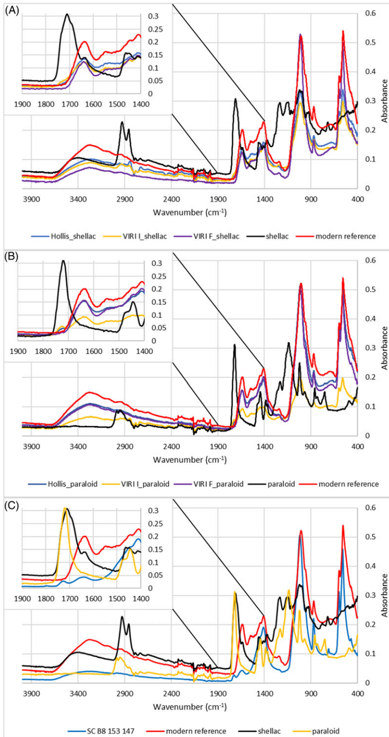
Figure 1 FTIR-ATR spectra of the bone samples contaminated with shellac (A) and Paraloid B-72 (B), and the Santa Catalina bone (SC B8 153 147) (C). The insets show the spectra around the peak at 1725 \text{cm}^{-1} .
