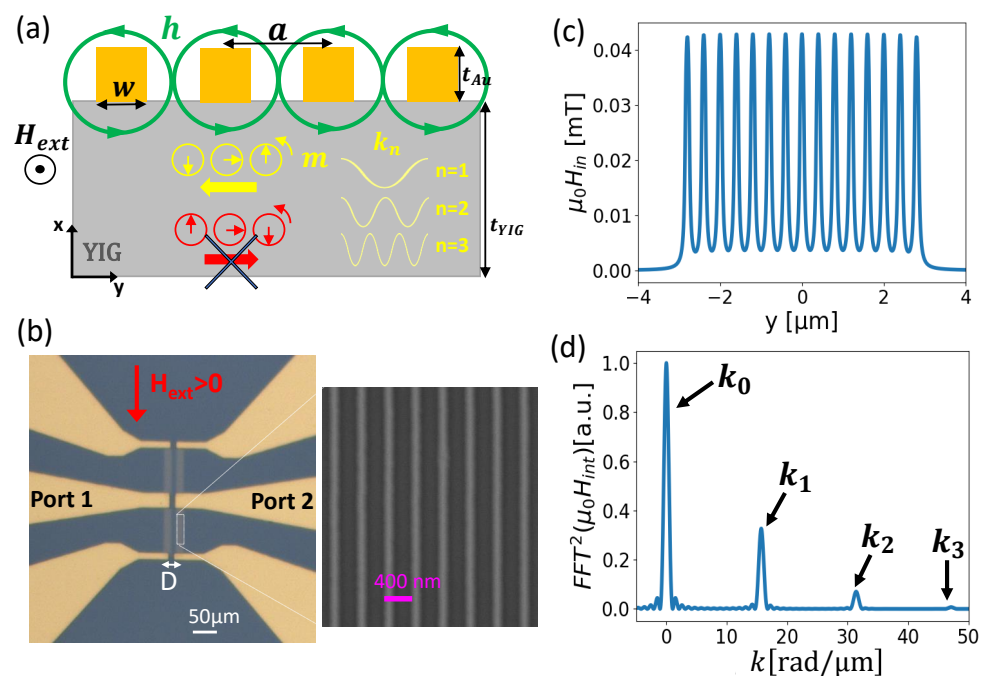
Figure 1. (a) Sketch of chiral excitation of SW from an Au nanowire grating. Green circle represents the microwave field h of Au NW, yellow and red circle represents the magnetization dynamics m respectively for left and right propagating direction. (b) Optical microscope image of the Au nanowire-grating sample. (c) Distribution of the in-plane microwave field. (d) Fourier transform of the in-plane exciting field.
