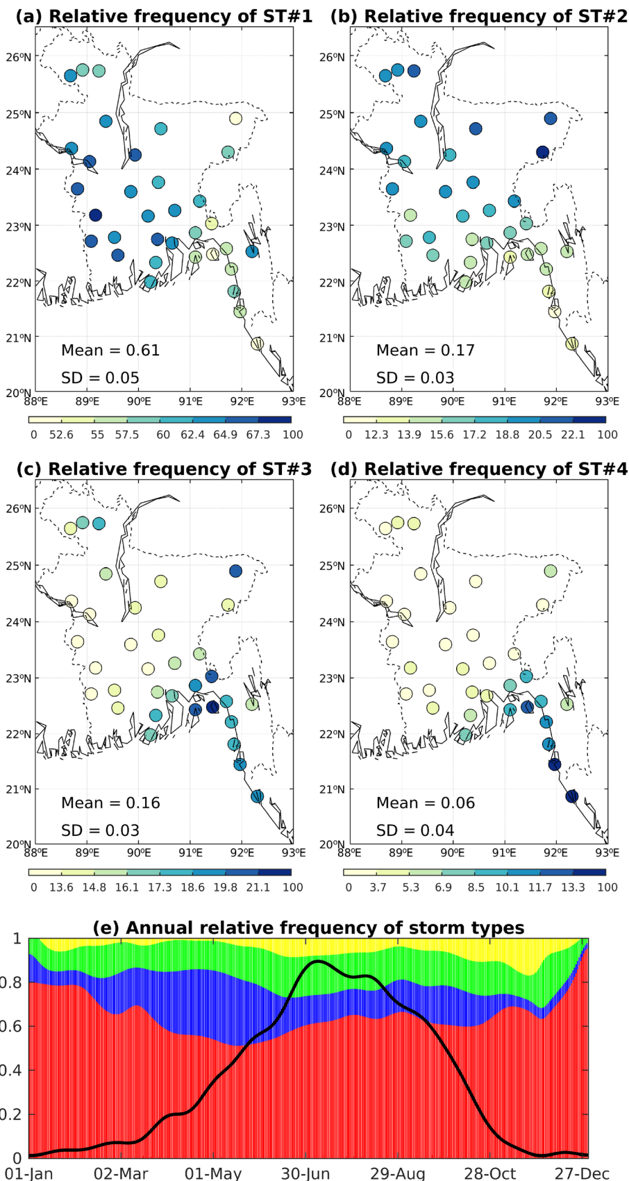
FIGURE 5 (a–d) Relative frequency of storm types (ST) #1–#4 with spatial average and standard deviation (SD) across the 34 stations shown in the lower left corner of each map. (e) Daily relative frequency of STs (displayed with the same colour as in Figure 4). The black line is the relative daily frequency of all STs considered together across the 34 stations (a value of 1 means that all stations receive at least 1 mm/3 hr all years. All time series in panel (e) are daily averages low pass filtered with a cut-off at 1/30 cycle-per-day [Colour figure can be viewed at wileyonlinelibrary.com ]
