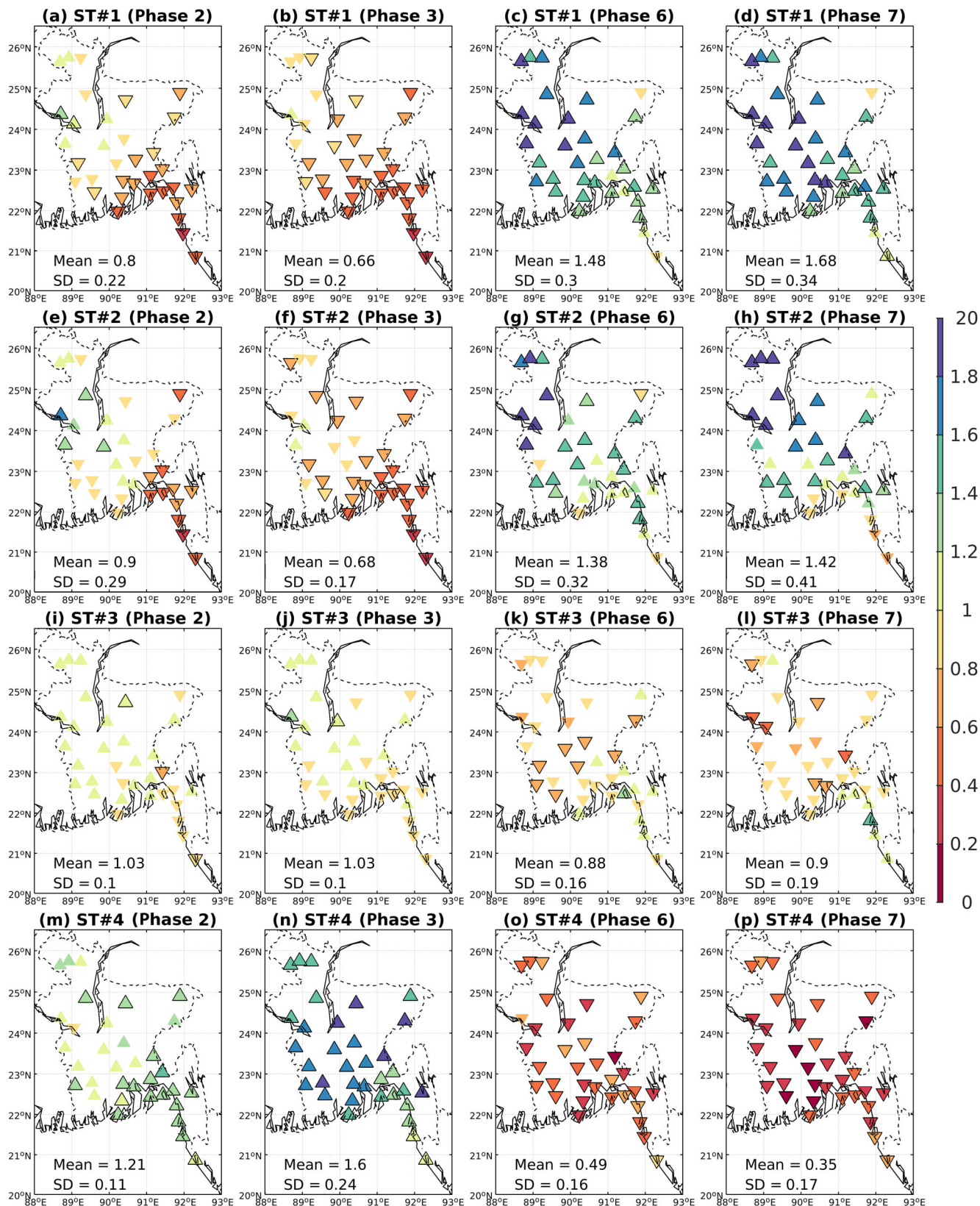
FIGURE 12 Local relative RR of the probability of occurrence of each ST in the Phases 2 (a,e,i,m) and 3 (b,f,j,n) and 6 (c,g,k,o) and 7 (d, h,l,p) of QBW defined in Figure 10c. The contoured upward (for RR > 1) and downward (for RR < 1) triangles indicate significant RR at the 99% level of significance. The spatial average and SD are indicated at the bottom of each map [Colour figure can be viewed at wileyonlinelibrary.com ]
