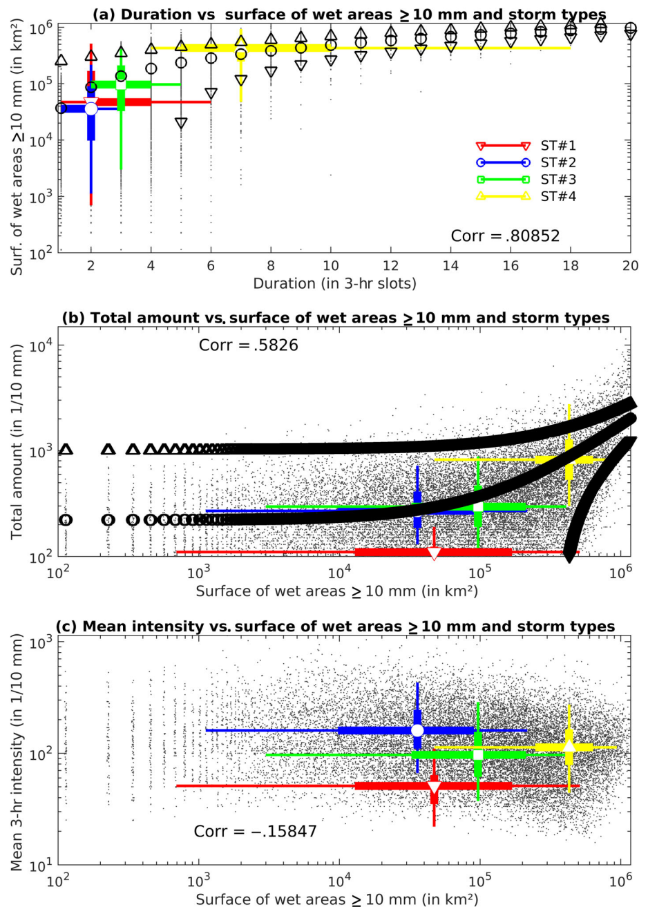
FIGURE 7 Same as Figure 4, except between the surface of IMERG wet area (in km 2 ) receiving at least 10 mm and (a) duration of wet events (WE) (in 3-hr slots), (b) total amounts (in 1/10 mm) and (c) mean intensity (in 1/10 mm per 3 hr) at the target BMD rain gauges. The sample is here reduced to WEs receiving at least 10 mm at the BMD rain gauge and at the co-located IMERG grid-points. Note that the linear fit line is not indicated on panel (c) because the common variance is <2% [Colour figure can be viewed at wileyonlinelibrary.com ]
