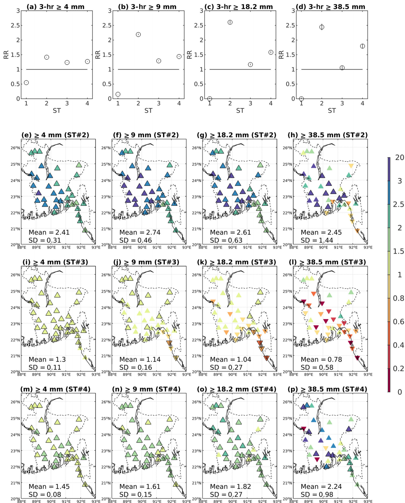
FIGURE 8 (a–d) Relative RR (dots with vertical line showing the 99% confidence interval) of probability of occurrence in each ST across all stations of 3-hourly rain \geq 4, 9, 18.2 and 38.5 mm. The RR is computed by stations on panels (e–h) for ST#2, panels (i–l) for ST#3 and (m–p) for ST#4. The spatial average and SD of RR are indicated at the bottom of each panel. Contoured upward (for RR > 1 ) and downward (for RR < 1 ) triangles indicate anomalous significant RR at the 99% level [Colour figure can be viewed at wileyonlinelibrary.com ]
