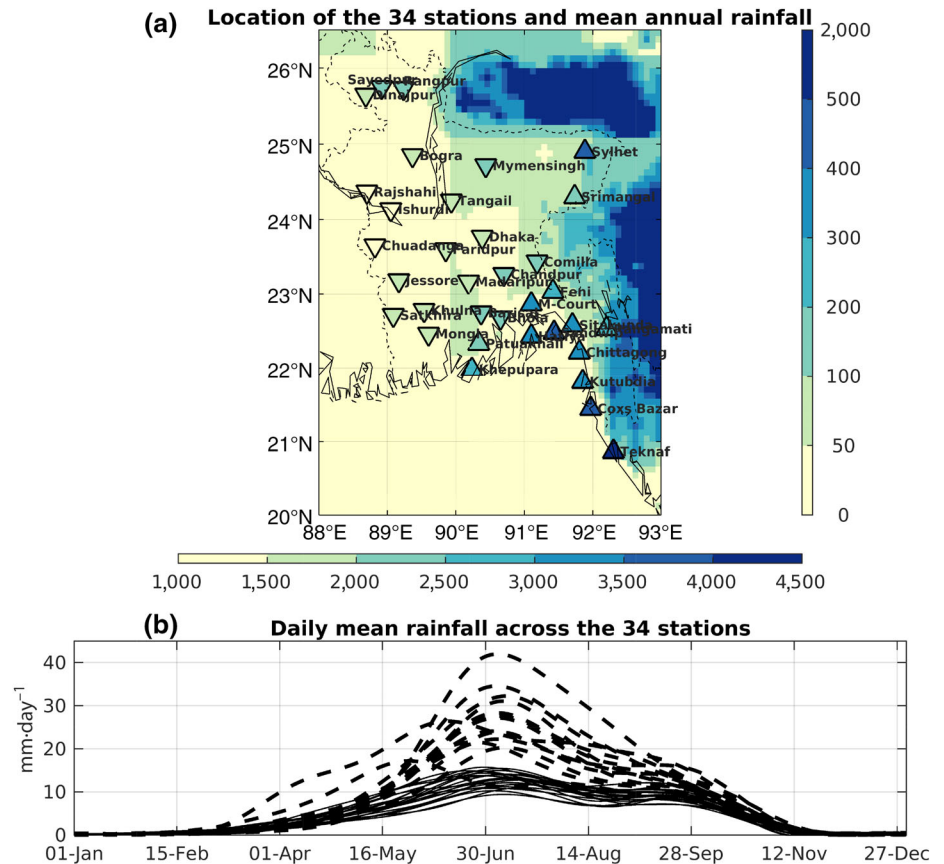
FIGURE 1 (a) Location of the 34 stations superimposed over the topography (shadings in metres above sea level, right legend) and with the mean annual rainfall (in millimetres, bottom legend) coded as upward and downward triangles. (b) Daily mean rainfall across the 34 stations averaged over the 22 years and low-pass filtered with a Butterworth's recursive filter with a cut-off at 1/60 cycle-per-day. The dashed lines show the stations with an upward triangle in (a) and the full lines show the stations with a downward triangle in (a) [Colour figure can be viewed at wileyonlinelibrary.com ]
