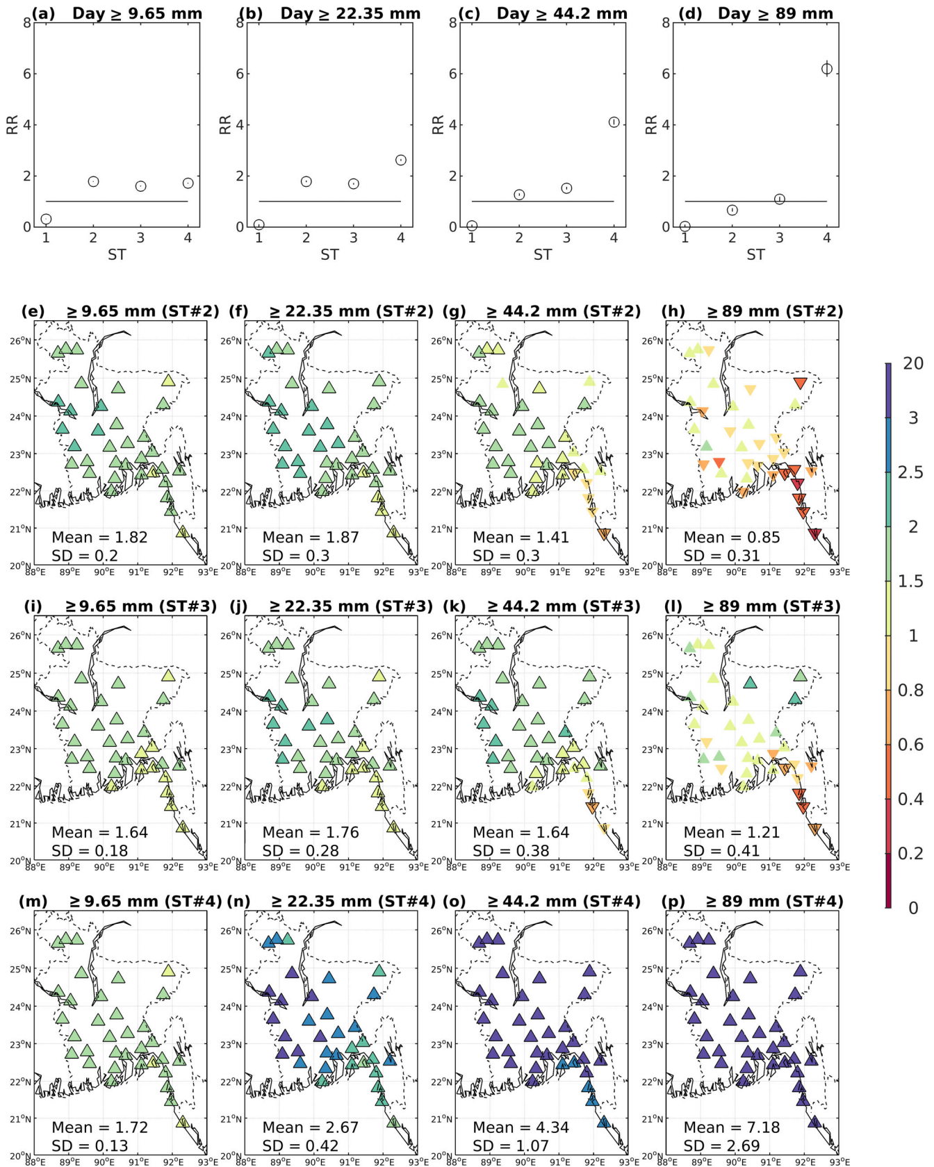
FIGURE 9 Same as Figure 8 except for daily rainfall \geq 9.65, 22.35, 44.20 and 89 mm. These thresholds are used by BMD to define respectively moderate, heavy moderate, heavy and very heavy daily rainfall [Colour figure can be viewed at wileyonlinelibrary.com ]
